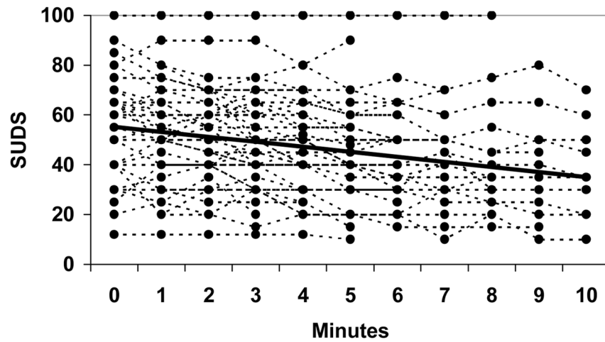
Figure 3. Third Exposure Observed Data and Average Fitted Growth Trajectory for Each Class
