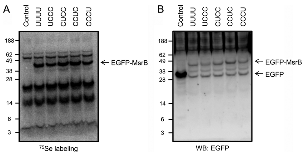
FIGURE 3. Insertion of four Sec residues into M. senile MsrB. A, HEK 293 cells expressing EGFP alone (Control), wild-type EGFP-MsrB with four Sec (UUUU), or single Sec-containing EGFP-MsrBs (UCCC, CUCC, CCUC, or CCCU) were labeled with ^{75}\text{Se} and analyzed by SDS-PAGE and PhosphorImager detection of ^{75}\text{Se} . EGFP-MsrBs (wild-type and Sec forms) were detected at \sim 43 kDa. B, expression of EGFP-MsrB confirmed by Western blotting (WB) using anti-GFP antibodies.
