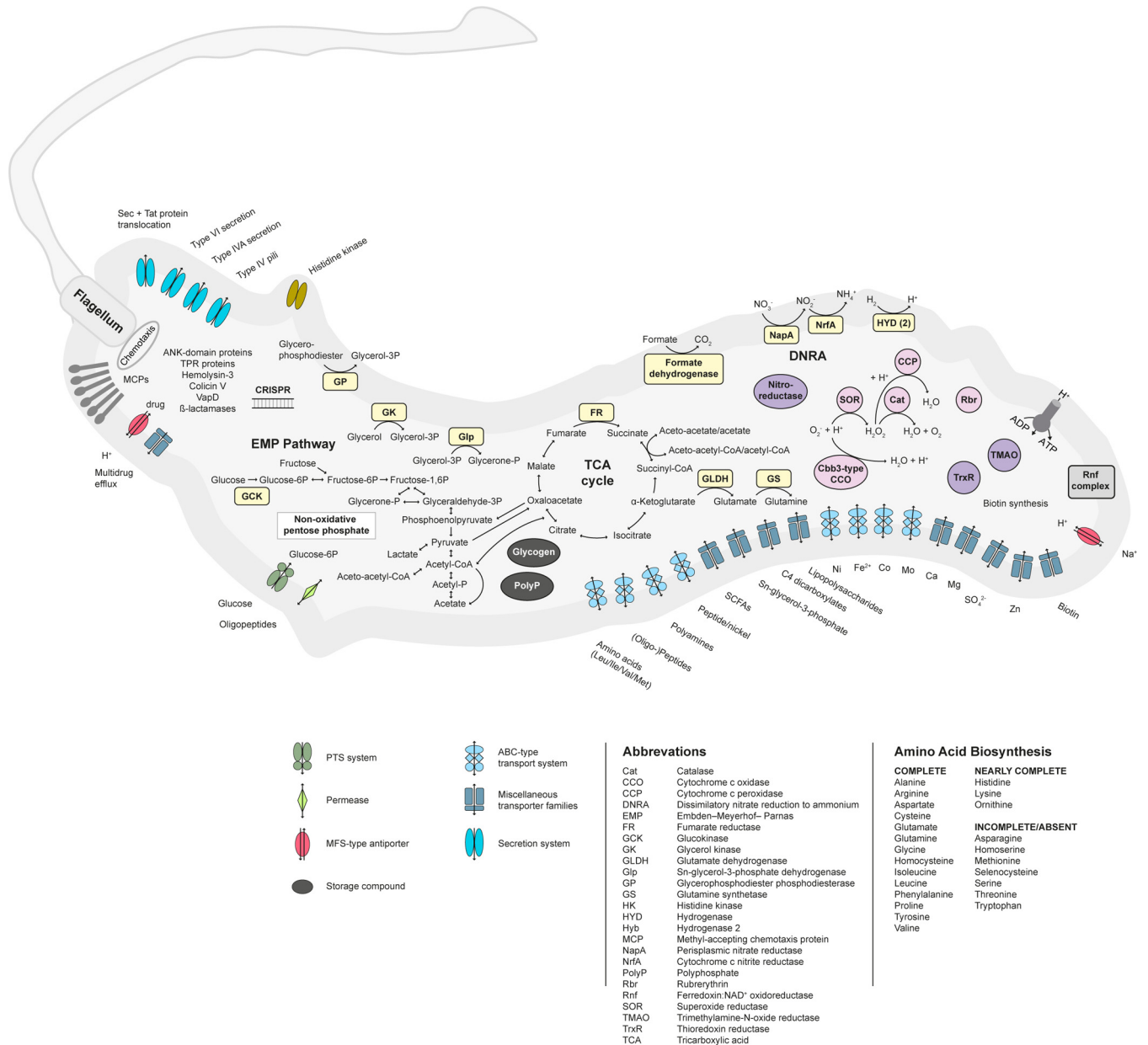
FIG 2 Selected genomic features of M. schaedleri ASF 457. Predicted metabolic and physiological capabilities based on genome annotations are shown.
