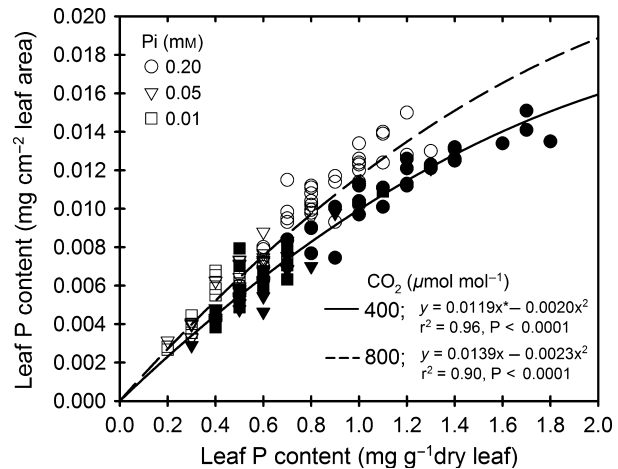
Fig. 4 Relationship between mass (mg g -1 leaf dry weight) and area bases (mg cm -2 leaf area) tissue P content in uppermost fully expanded cotton leaves grown at either ambient (filled symbols, 400 μmol mol -1 ) or elevated (unfilled symbols, 800 μmol mol -1 ) CO 2 under different phosphate (Pi) treatments. Data are from individual plants measured between 57 and 112 days after planting across two experiments. A polynomial second order equation was used, and intercept was forced to pass through origin (zero). The asterisk (*) indicated significant ( P < 0.05 ) difference in the linear term of the equations between two CO 2 levels.
