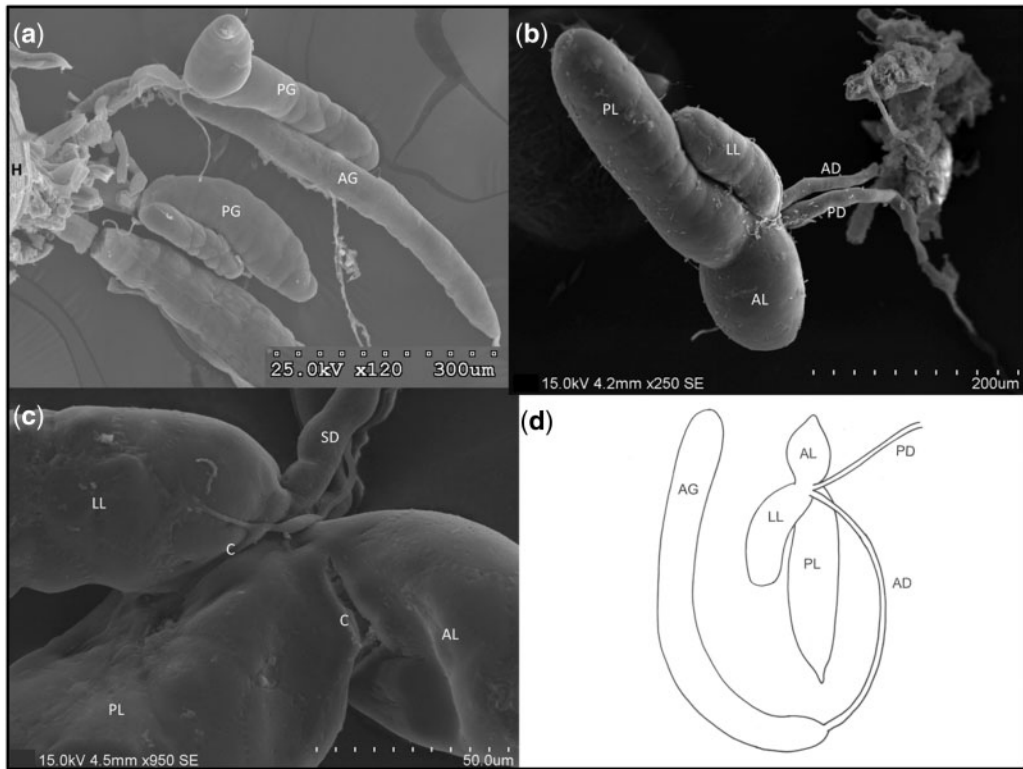
Fig. 2. Scanning electron micrograph images of the salivary glands of B. occidius : (a) complete salivary gland complex showing two principal glands (PG) and a connected accessory gland (AG) in proximity to the B. occidius head (H); (b) PG with the anterior (AL), posterior (PL), and lateral (LL) lobes and the associated principal (PD) and accessory gland (AD) ducts; (c) PG with AL, PL, and LL lobes and constrictions (C) between the lobes and associated salivary duct (SD). Scale bars are shown at the bottom right corner of each image. (d) Schematic drawing of one half of the B. occidius salivary gland pair. Principal gland is composed of the anterior lobe (AL), lateral lobe (LL), and posterior lobe (PL). Accessory gland (AG), accessory gland duct (AD), and principal gland duct (PD) are also shown.
