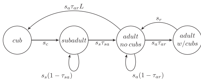
Fig. 1. Four stage classes in the female black bear life cycle are represented by circles; arrows indicate possible transitioning between stages or staying in the same stage class; s_i are survival probabilities for stage i : s_c (cubs), s_s (subadults), s_a (adults available to breed), and s_r (adults with cubs); \tau_i are transition probabilities \tau_{sa} (subadults to adults without cubs) and \tau_{ar} (adults without cubs to adults with cubs); L is the average number of female cubs per litter.
