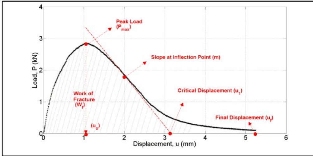
Figure 2-8 Calculation of the post peak slope (Al-Qadi, Ozer et al. 2015)
