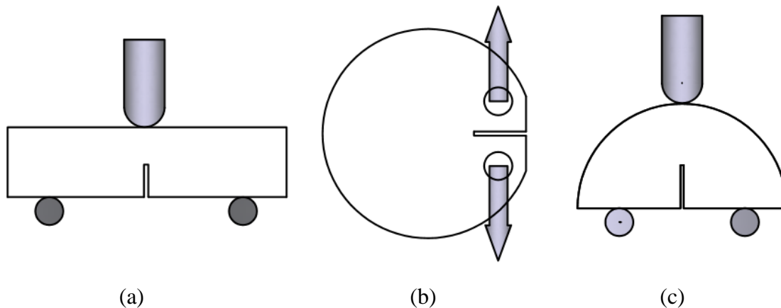
Figure 2-1 Fracture tests for asphalt concrete mixtures: (a) single-edge notched beam (SEB) test, (b) disk-shaped compact tension (DCT) test, and (c) semicircular bending (SCB) test.
