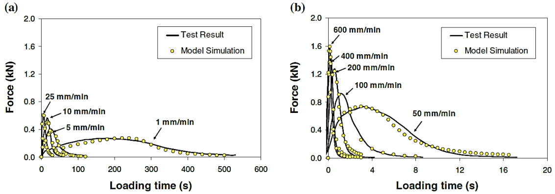
Figure 2-3 Effect of loading rate (Aragão and Kim 2012).
