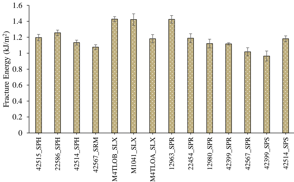
Figure 5-4 SCB test results (fracture energy) of different mixtures with standard error bars
