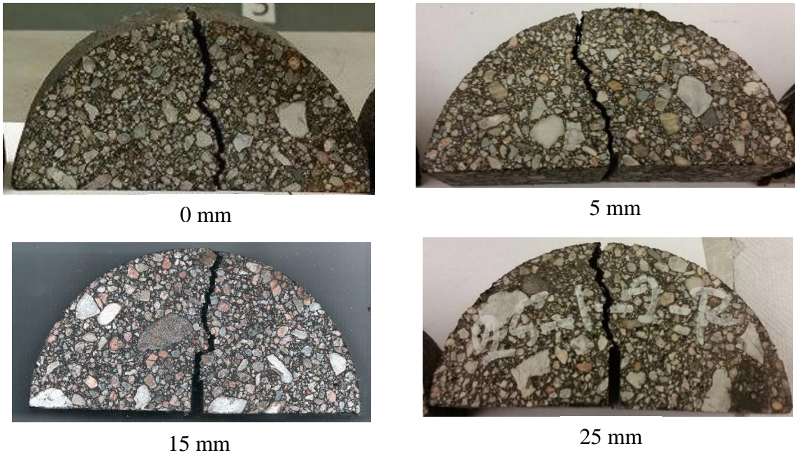
Figure 4-6 Fracture profile at different notch lengths
