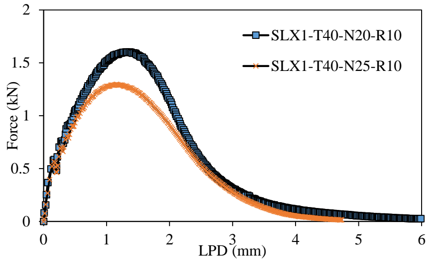
Figure 2-6 Calculating critical J-Integral using two notches
