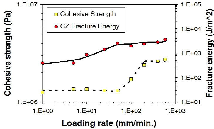
Figure 2-4 Numerical simulation results of SCB fracture testing at different loading rates by Aragón and Kim (2012).
