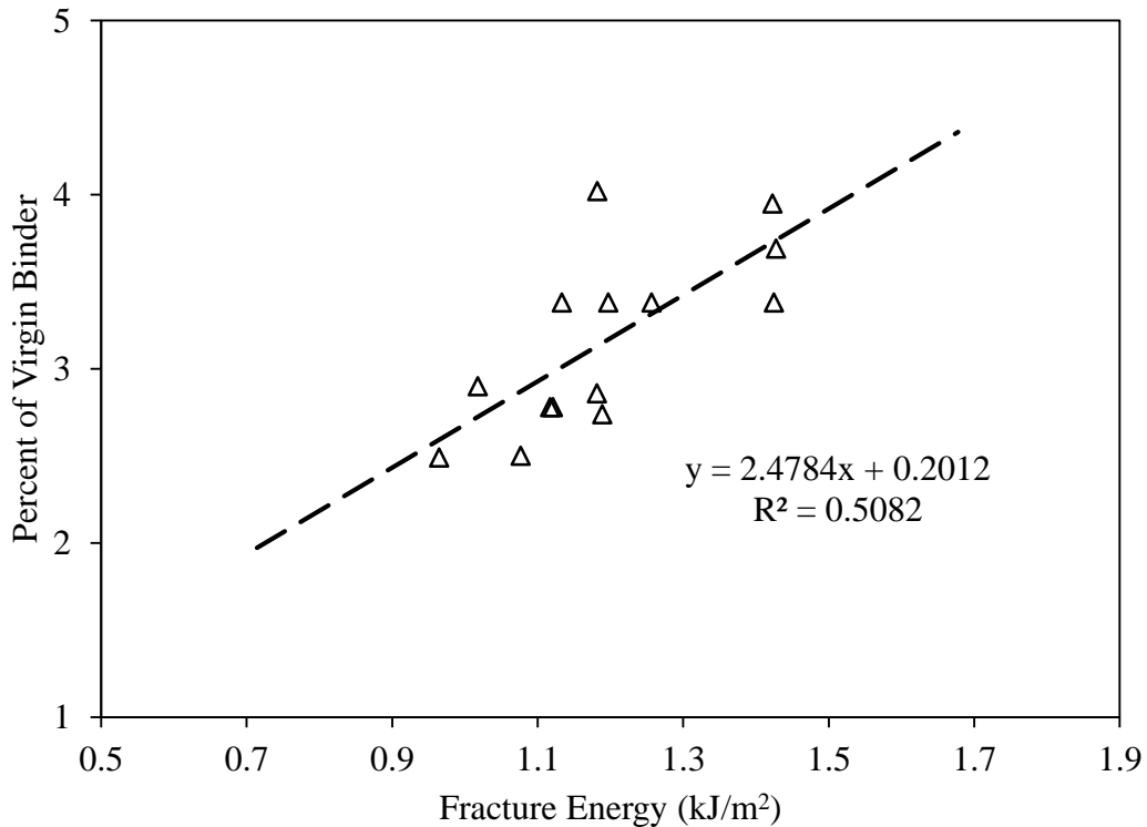
Figure 5-6 Relationship between virgin binder and fracture energy
