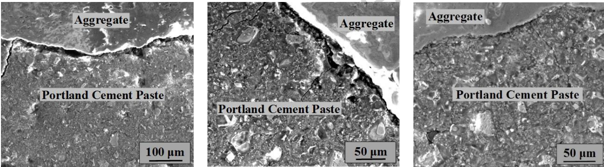
Fig. 2. SEM images of interphases in PCC
