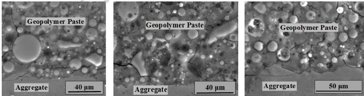
Fig. 3. SEM images of interphases in GPC
