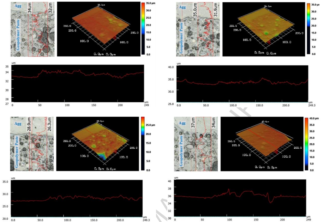
Fig. 6. Topography LSM images of aggregate-paste in GPC
