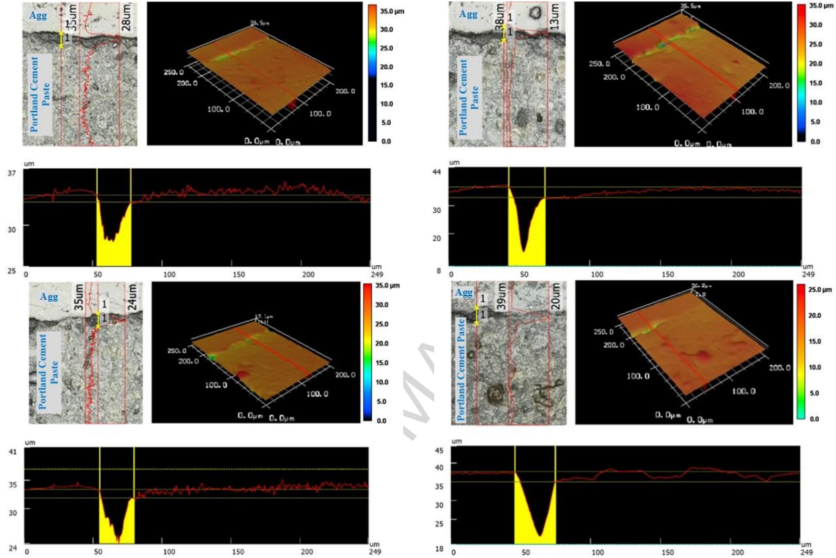
Fig. 4. Topography LSM images across aggregate-paste in PCC
