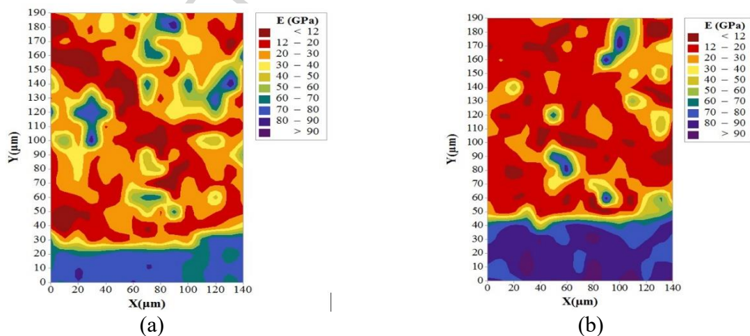
Fig. 8. Contour maps of elastic modulus (GPa), (a) GPC, (b) PCC
