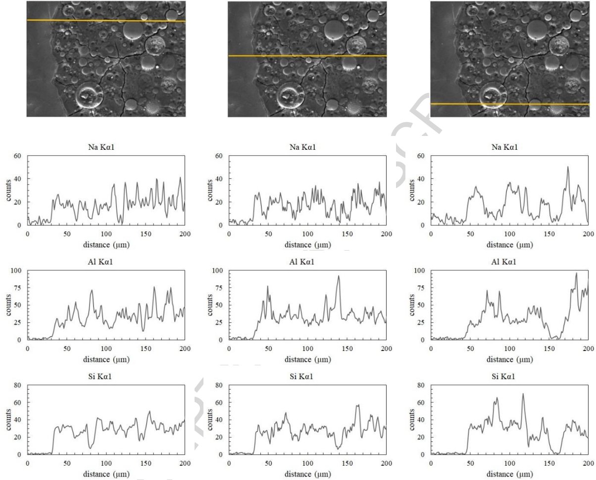
Fig. 12. SEM-EDX line scan across aggregate-paste in GPC
