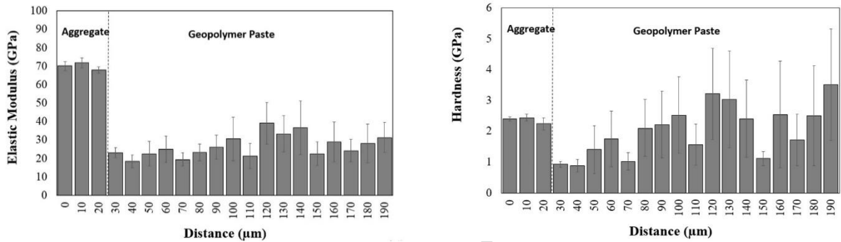
Fig. 9. Grid indentation modulus and hardness across aggregate-paste in GPC
