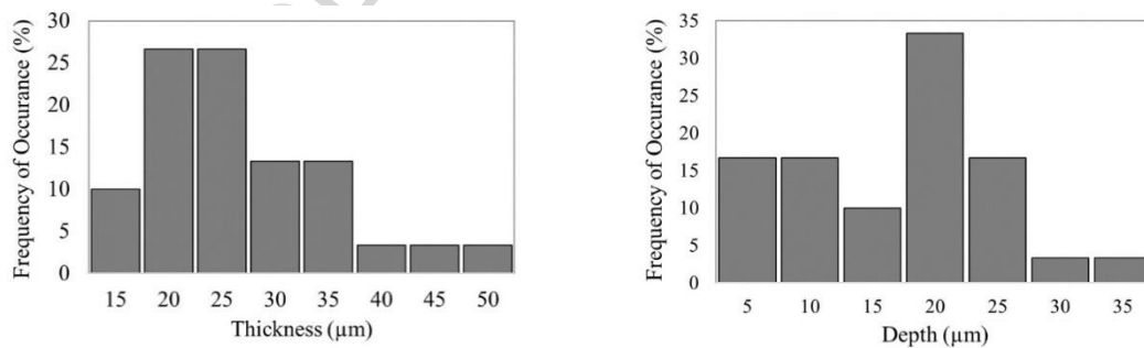
Fig. 5. Frequency distribution of thickness and depth of interfacial debonding
