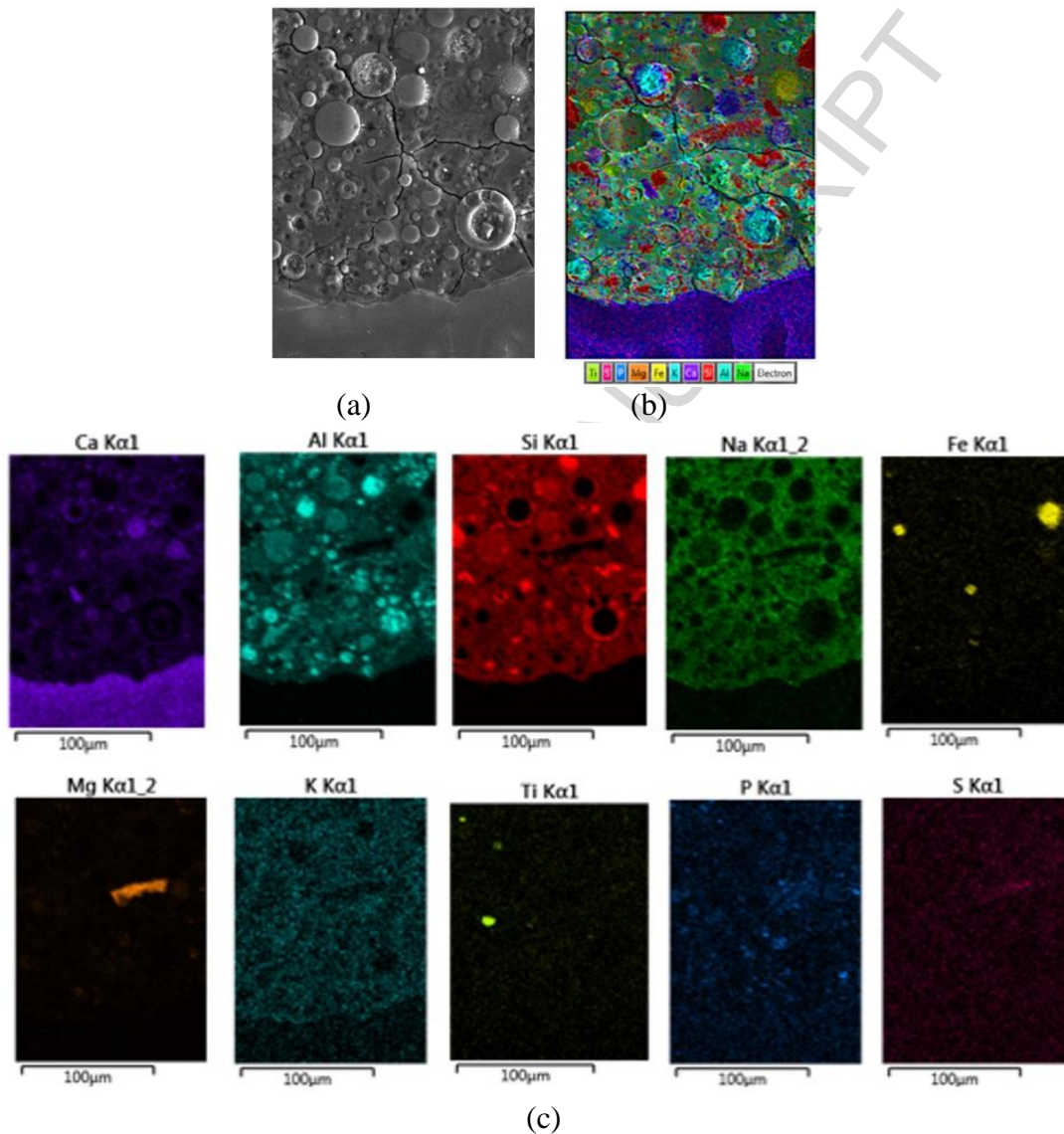
Fig. 11. Qualitative EDS map analysis of GPC mixture, (a) SEM image, (b) overlay map, (c) individual elemental maps.
