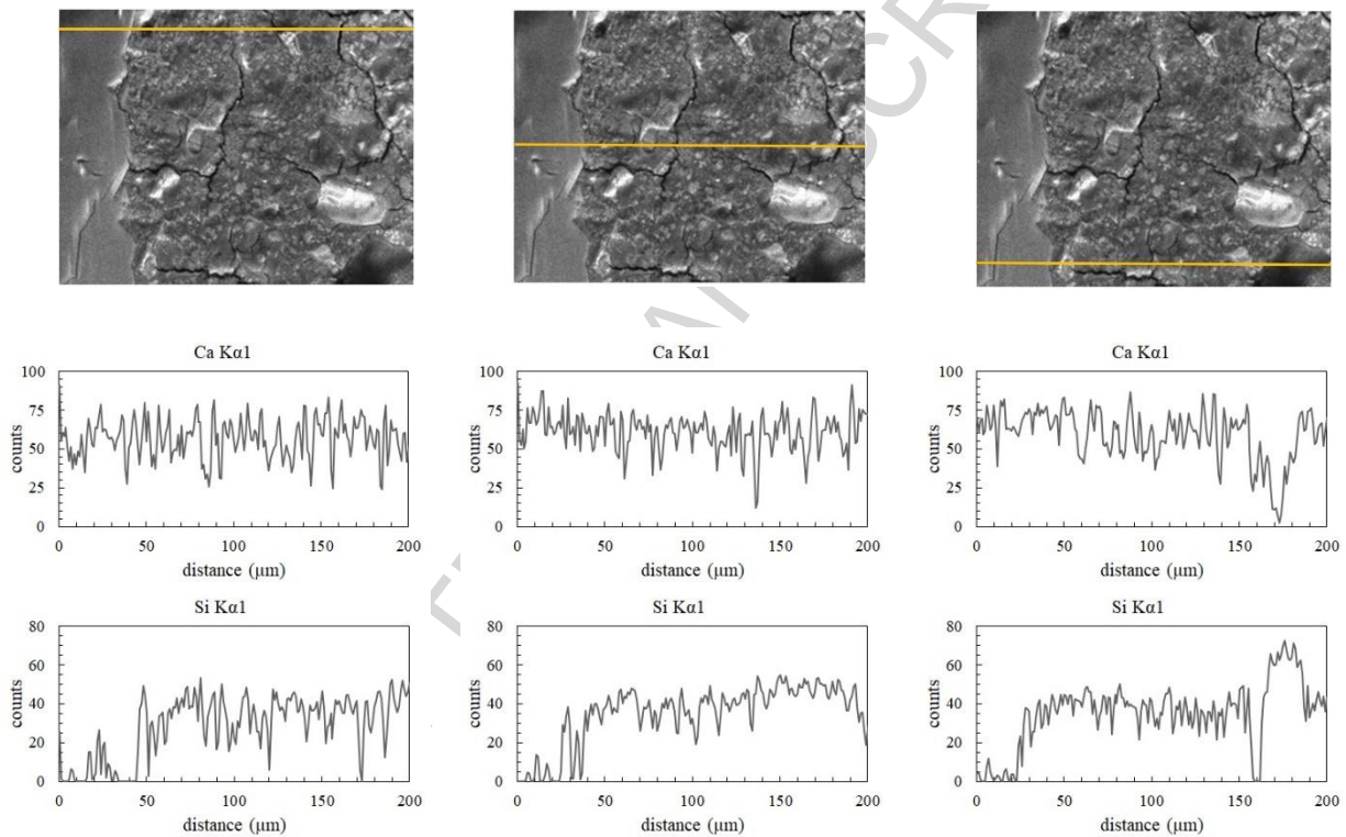
Fig. 14. SEM-EDX line scan across aggregate-paste in PCC
