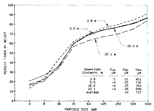
Fig. 8—Size distributions of eroded sediment from interrill areas at selected downslope distances for corn residue rate of 1.12 t/ha. The sediment sizes listed in the lower right table are those for which 16, 50 or 84%, respectively, of the sediment was smaller.
