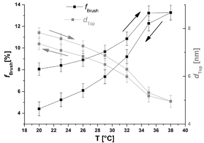
Figure 5. Results of the best-match model calculation of GE measurements of temperature induced swelling and deswelling of PNIPAAm brushes on STFs.
