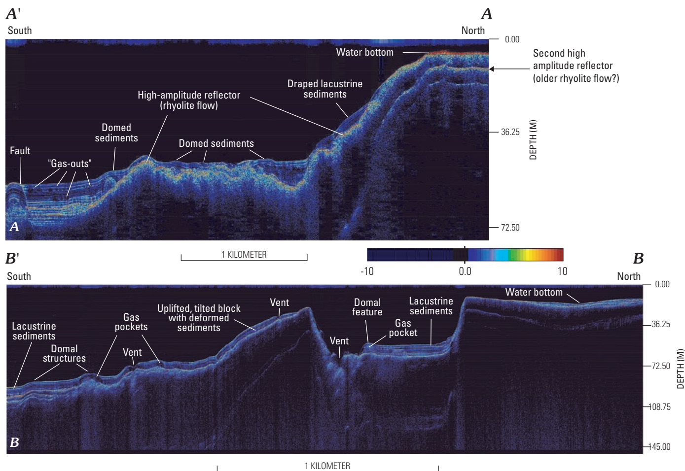
Figure 4. High-resolution seismic-reflection images. A , High-resolution seismic-reflection image from northwestern West Thumb basin showing high-amplitude (discontinuous red and yellow) reflector interpreted as a sub-bottom rhyolitic lava flow. Glacial and lacustrine sediments, marked in blue, overlie this unit. The data amplitudes have been debiased and spatially equalized only; no additional gain corrections or filtering were applied. B , High-resolution seismic-reflection image (line YL72) across part of Elliott's explosion crater showing small vents, gas pockets, and domed sediments in the lacustrine sediments that overlie the crater flank. Lacustrine-sediment thickness in the main crater indicates 5–7 thousand years of deposition since the main explosion. More recent explosions, in the southern part of the large crater, ejected postcrater lacustrine sediments and created new and smaller craters. Colors are the same as for figure 4A.
