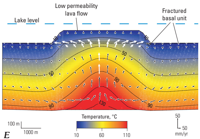
Figure 10. Flow model for hydrothermal vents and rhyolitic lava flows in Yellowstone Lake. A , Schematic diagram showing physical features of a rhyolitic lava flow (modified from Bonnichsen and Kauffman, 1987). B , Two-dimensional fluid-flow model with simple glaciolacustrine-sedimentary aquifer (no caprock) that results in low flow velocities, recharge at the surface, and lateral flow out of both ends of the model aquifer. Subsurface temperatures never exceed 114°C, as indicated by contours and color map. Fluid-flow rates are low (<0.7 mm/yr) as indicated by velocity vectors. C , Fluid-flow model with a fully cooled rhyolitic lava flow acting as caprock. The
