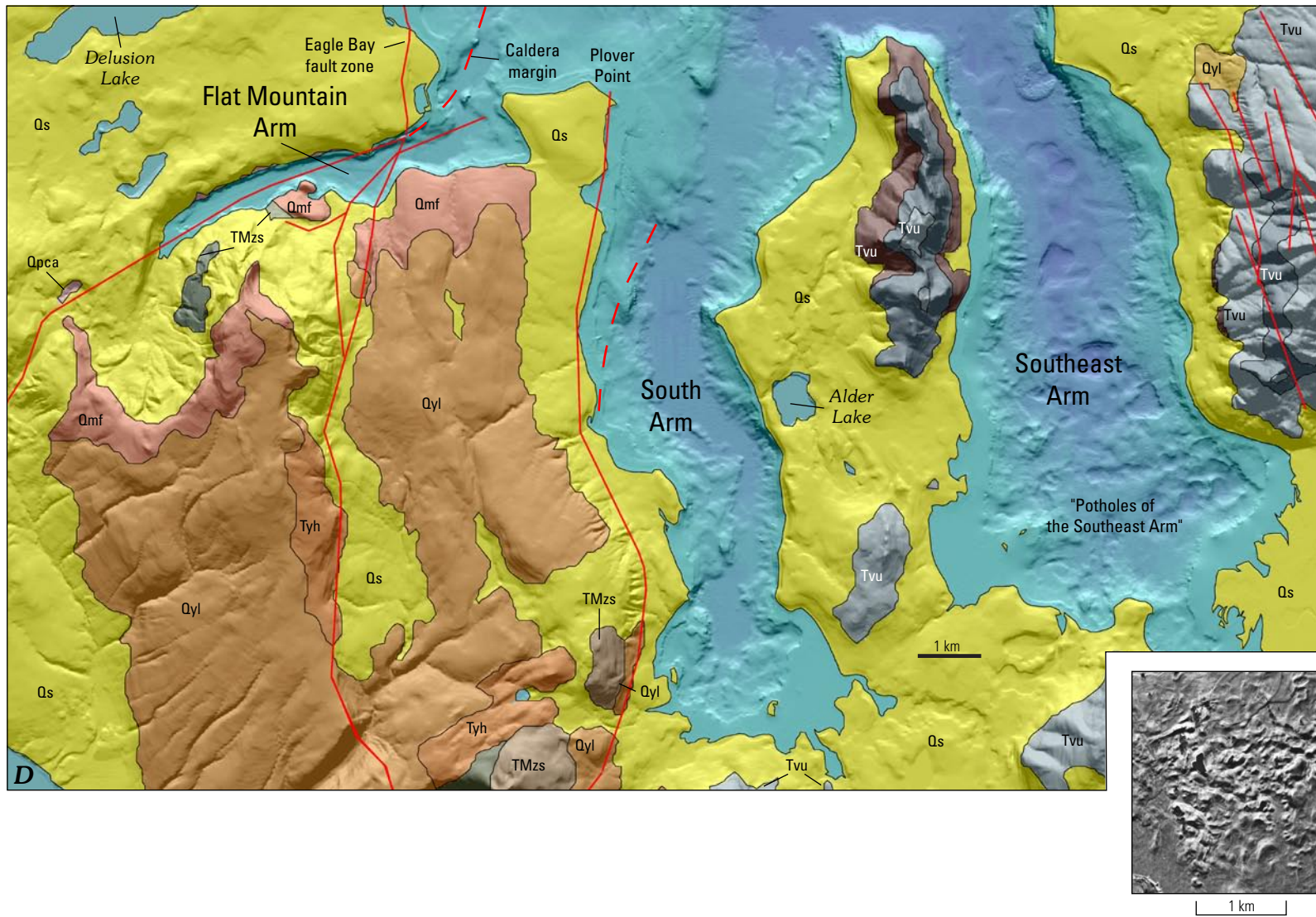
D , High-resolution bathymetric map of the South, Southeast, and Flat Mountain Arms, acquired by multibeam-sonar imaging in 2002, showing the glaciated landscape of the lake floor in the southernmost part of Yellowstone Lake and several faults. The bathymetry in the Southeast Arm contains many glacial-meltwater and stagnant-ice-block features; the area, informally referred to as the “Potholes of the Southeast Arm,” resembles much of the kettle-dominated topography mapped by Ken Pierce and others in Jackson Hole, Wyo. See fig. 1B for descriptions of geologic units. The inset is a gray-shaded-relief map of “The Potholes” in Jackson Hole. Image from Good and Pierce (1996).
