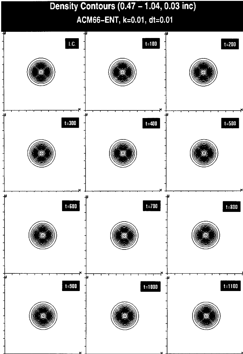
FIG. 4.1.12. Convecting vortex: Comparison of ACM66-ENT with the exact solution (I.C.), illustrated by density contours at t = 100, 200, 300, 400, 500, 600, 700, 800, 900, 1000, 1100 for \Delta t = 0.01 and \kappa = 0.01 on a 80 \times 79 grid.
