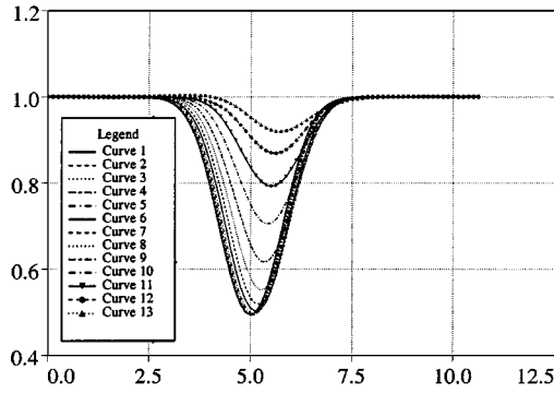
FIG. 4.1.5. Convecting vortex: Comparison of ACM66-ENT with the exact solution (left-most solid line), illustrated by density profiles at the centerline y=0 , at t = 100, 200, 300, 400, 500, 600, 700, 800, 900, 1000, 1100, 1200 for \Delta t = 0.02 and \kappa = 0.01 on a 80 \times 79 grid. The left-most solid curve is the exact solution and the rest of the curves shifted to the right are the corresponding time sequences in an increasing order.
