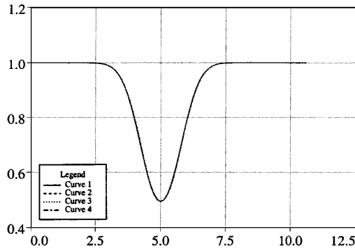
FIG. 4.1.7. Convecting vortex: Comparison of ACM66S-ENT with the exact solution (solid line), illustrated by density profiles at the centerline y=0 , at t = 100, 200, 300 (curves 2–4) for \Delta t = 0.01 and \kappa = 0.005 on a 80 \times 79 grid.
