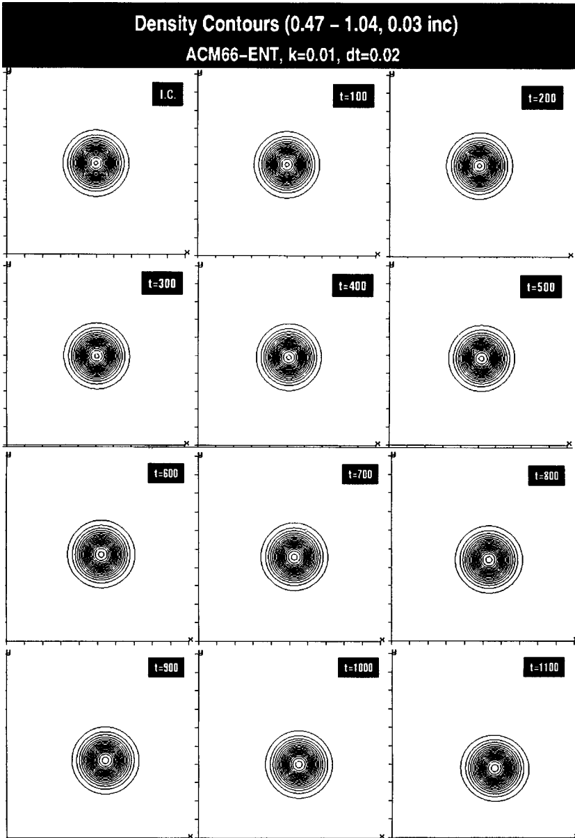
FIG. 4.1.11. Convecting vortex: Comparison of ACM66-ENT with the exact solution (I.C.), illustrated by density contours at t = 100, 200, 300, 400, 500, 600, 700, 800, 900, 1000, 1100 for \Delta t = 0.02 and \kappa = 0.01 on a 80 \times 79 grid.
