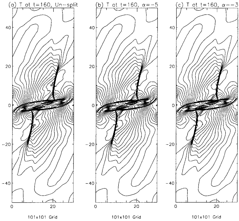
FIG. 4.2.3. Vortex pairing: Comparison of normalized temperature contours for \alpha = -5 and -3 with the un-split approach at time t = 160 on a 101 \times 101 grid with \kappa = 0.7 for the nonlinear fields and \kappa = 0.35 for the linear fields using ACM66.
