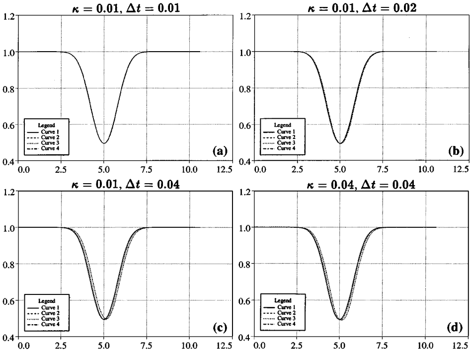
FIG. 4.1.4. Convecting vortex: Comparison of ACM66-ENT with the exact solution (solid line), illustrated by density profiles at the centerline y = 0 , at t = 100, 200, 300 (curves 2–4) for \Delta t = 0.01, 0.02, 0.04 and \kappa = 0.01 , and for \Delta t = 0.04 and \kappa = 0.04 on a 80 \times 79 grid.
