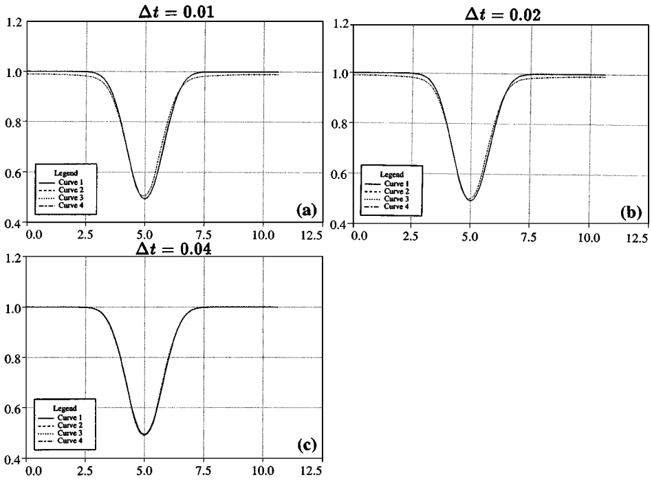
FIG. 4.1.3. Convecting vortex: Comparison of ACM66 with the exact solution (solid line), illustrated by density profiles at the centerline y = 0 , at t = 100, 200, 300 (curves 2–4) for \Delta t = 0.01, 0.02, 0.04 , \kappa = 0.06 on a 80 \times 79 grid.
