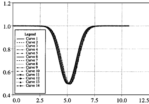
FIG. 4.1.6. Convecting vortex: Comparison of ACM66-ENT with the exact solution (left-most solid line), illustrated by density profiles at the centerline y=0 , at t = 100, 200, 300, 400, 500, 600, 700, 800, 900, 1000, 1100, 1200, 1300 for \Delta t = 0.01 and \kappa = 0.01 on a 80 \times 79 grid. The left-most solid curve is the exact solution and the rest of the curves shifted to the right are the corresponding time sequences in an increasing order.
