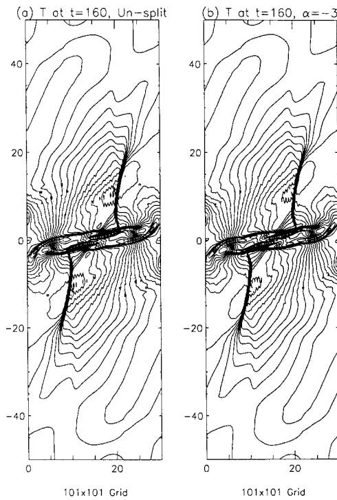
FIG. 4.2.4. Vortex pairing: Comparison of normalized temperature contours for \alpha = -3 with the un-split approach at time t = 160 on a 101 \times 101 grid with \kappa = 0.7 for the nonlinear fields and \kappa = 0 for the linear fields using ACM66.
