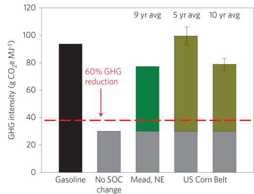
Figure 3. Contribution of modelled \text{CO}_2 emissions from SOC to the life cycle of biofuel from corn residue. Error bars are \pm one standard deviation, based on Figure 2c. Data are also from Figure 1 and Supplementary Tables 7 and 8.
