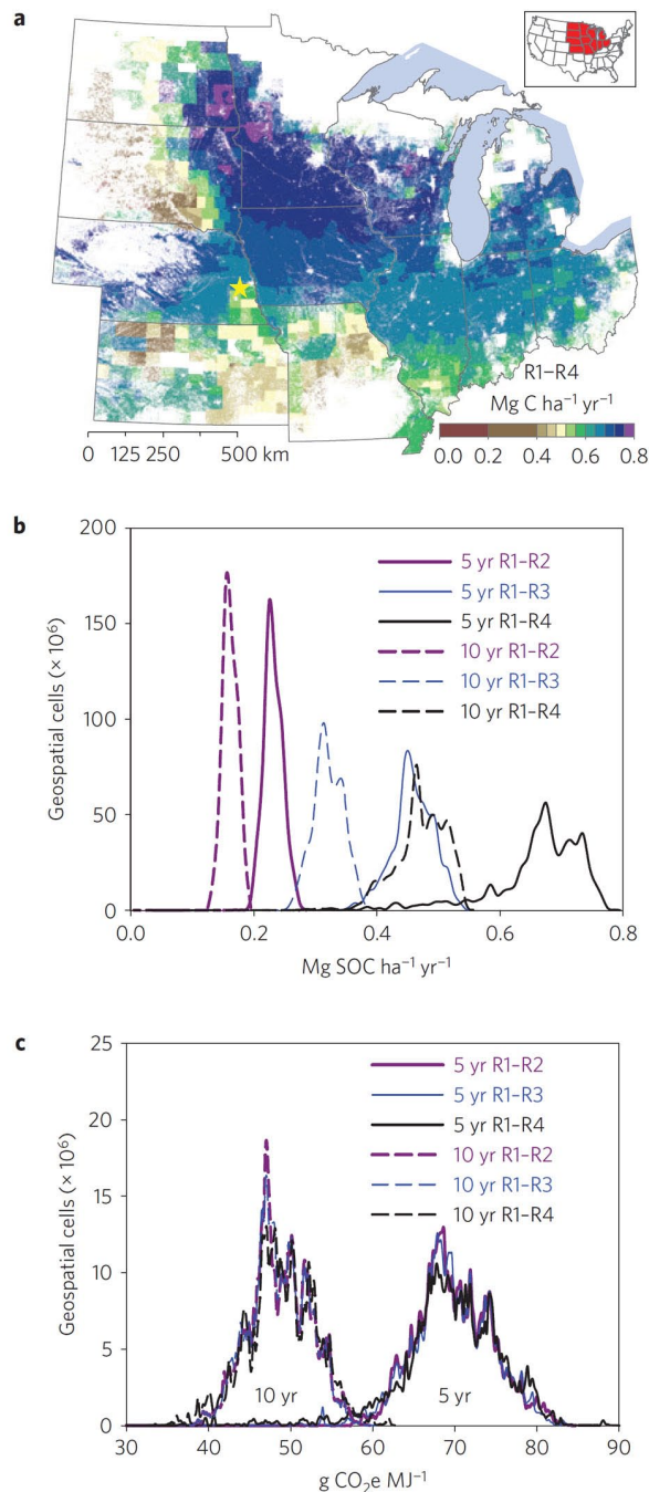
Figure 2. Modelled soil organic carbon respiration to \text{CO}_2 in the US Corn Belt from corn residue removal. a) Geospatial modelling of soil organic carbon (SOC) loss from 6 \text{ Mg ha}^{-1} \text{ yr}^{-1} of residue removal (first five years) relative to no removal (580 million cells; Mead, Nebraska, is indicated). b) Loss of SOC compared with no removal by removal level and time. c) \text{CO}_2 emissions increase in the biofuel life cycle corresponding to b .
