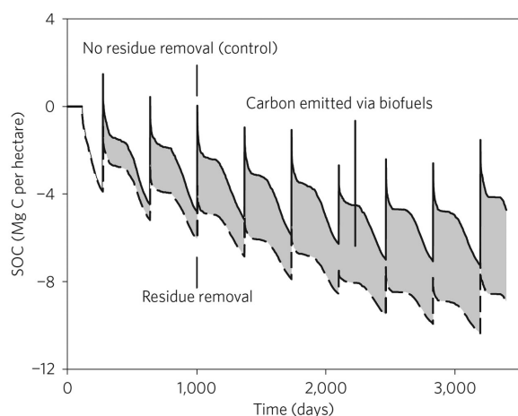
Figure 1. Modelled soil organic carbon decrease due to removal of 6 Mg corn residue per hectare per year over nine years compared with no removal under irrigated continuous corn. Daily modelled oxidation of soil organic carbon (SOC) and residue to CO 2 is based on field measurements of initial SOC (0–30 cm soil depth), corn residue input, and temperature at Mead, Nebraska. The average annual net loss of SOC is 0.47 Mg C ha -1 yr -1 , but declines exponentially from 1.13 to 0.25 Mg C ha -1 yr -1 over the first eight years.
