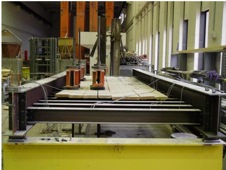
Figure 4-5. Two-Girder Bridge Setup
