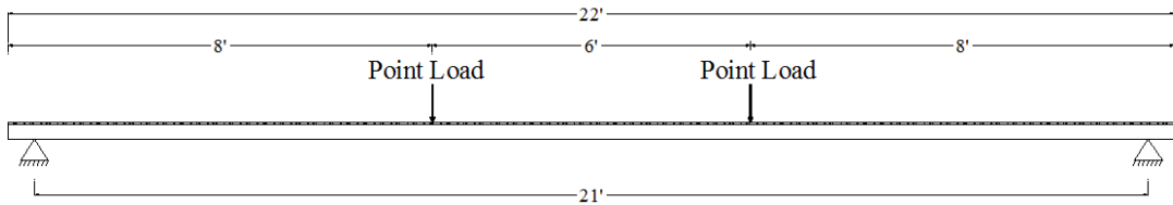
Figure 4-8. Longitudinal View of Loading Points in Experiment 1.
