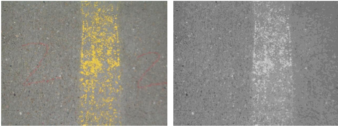
Figure 7.1. Actual picture (on left) and grayscale image (on right) of pavement after marking has been removed
