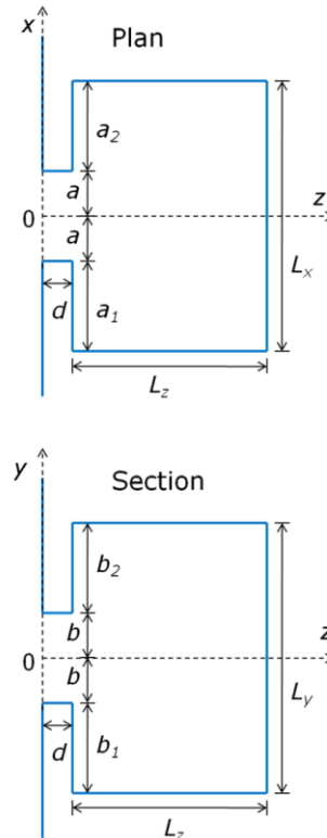
Figure 4. Geometry and dimensions of the present models
