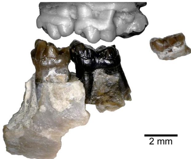
Fig. 4. Occlusion of upper and lower dentitions of Ekgmowechashala zancanelloi from Oregon, in lateral view. Illustrated above is the maxillary dentition of UCMP 128231 (grayscale cast) and below is the mandibular dentition of JODA 6322, both in lateral view. Scale bar equals 2 mm. [Color figure can be viewed in the online issue, which is available at wileyonlinelibrary.com .]
