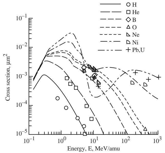
Figure 10. Calculations and experimental values of mutation cross sections versus energy for HPRT mutations in V79 cells. Data from Thacker, Stretch, and Stephens 1979; Kranert, Schneider, and Kiefer 1990; Belli et al. 1993; Kiefer, Stoll, and Schneider 1994.
