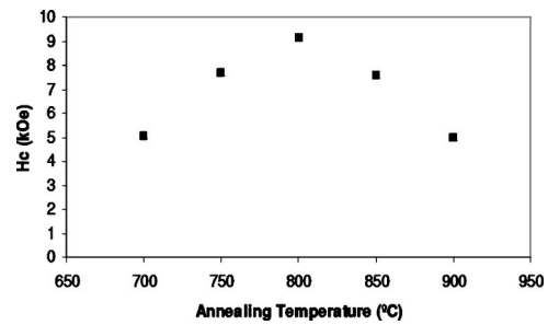
FIG. 2. Relationship between annealing temperature and intrinsic coercivity (for as-solidified ribbon H_c=4 kOe).
