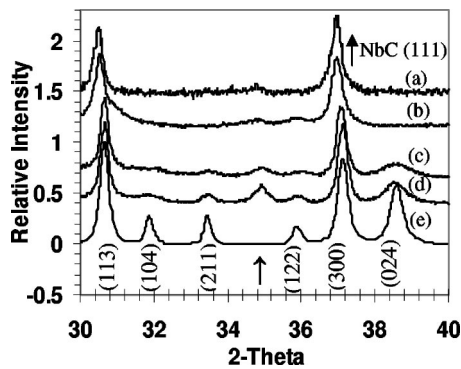
FIG. 1. X-ray diffraction scans of (a) the as-solidified Sm-Co-Nb-C alloy, and after heat treatment at (b) 750 °C, (c) 850 °C, and (d) 900 °C. (e) Calculated diffraction pattern for Sm 2 Co 17 .
