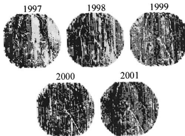
Fig. 4. Gray-scale yield maps of the 1997 through 2001 crop seasons from the Gibbon, NE, site. Variations in color, from dark to light, correspond to decreasing grain yields.
