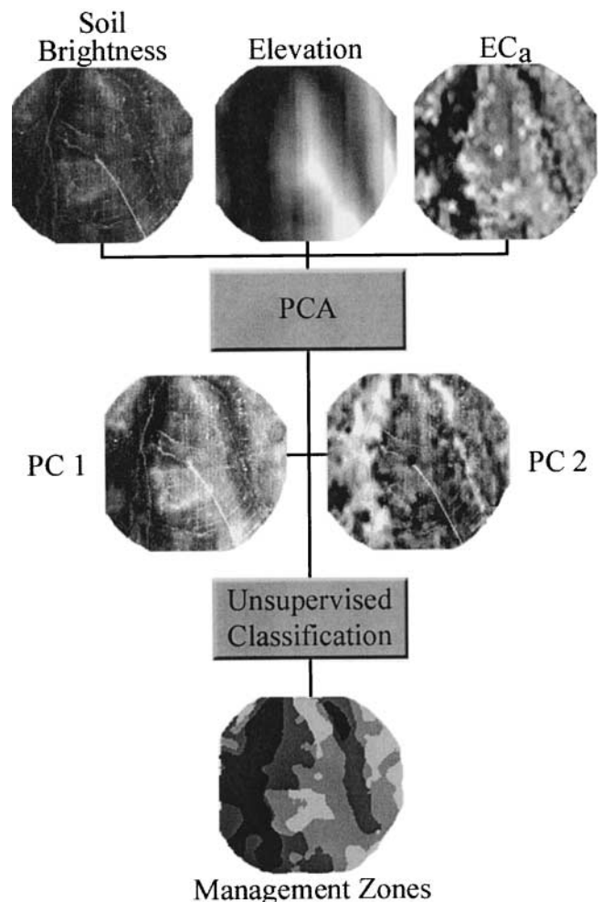
Fig. 2. (Top) Gray-scale maps of five landscape attributes acquired at the Gibbon, NE, corn study site consisting of red, green, and blue bands (shown in one map) of soil brightness image, elevation, and apparent electrical conductivity (EC a ), with variations in color, from dark to light, corresponding to increasing values for all landscape attributes. (Middle) Gray-scale maps of principal-component (PC) scores for PCs 1 and 2, resulting from principal-component analysis (PCA) of five landscape attributes, with variations in color, from dark to light, corresponding to decreasing PC scores. (Bottom) Gray-scale map of management zones (MZ), resulting from unsupervised classification of PC scores for two PCs, with variations in color, from dark to light, corresponding to MZ 1 through 4.
