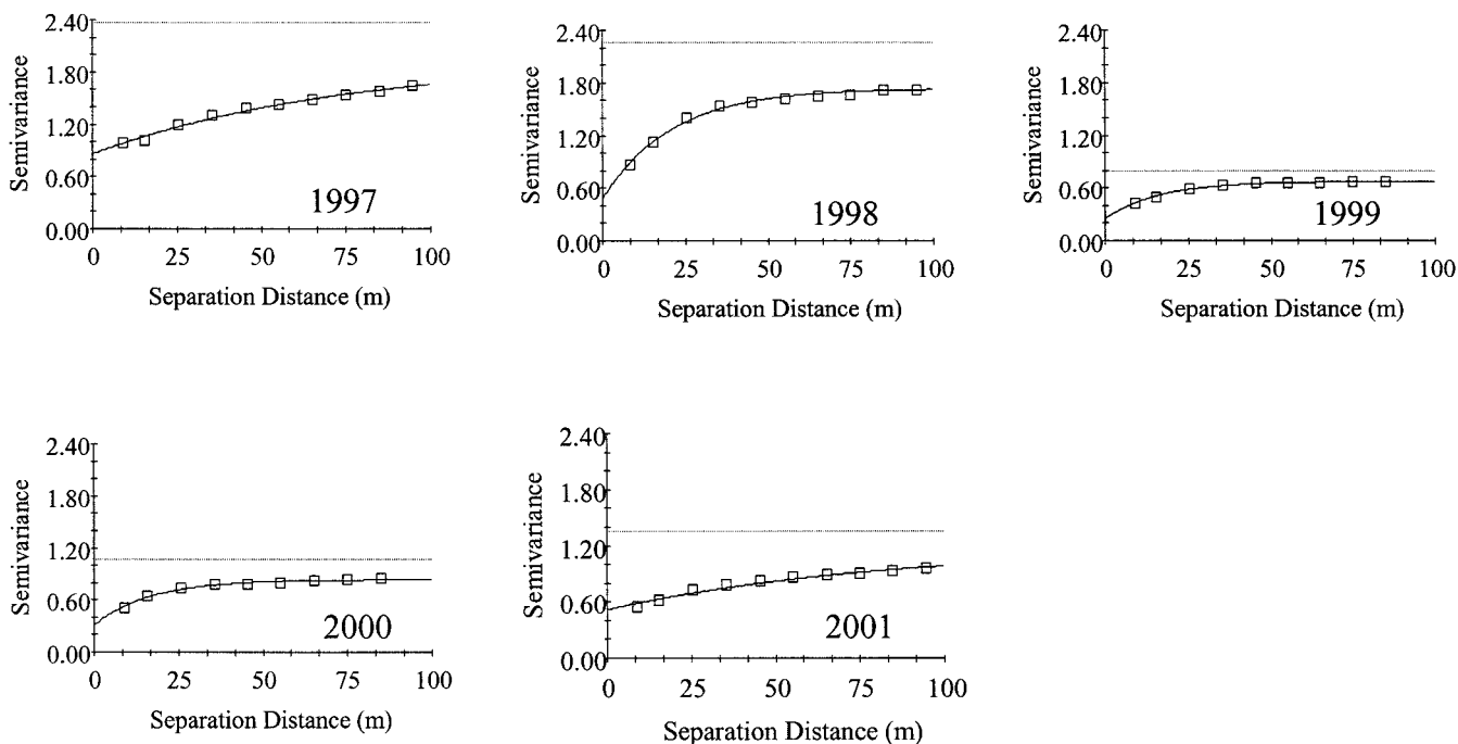
Fig. 5. Semivariance analysis of yield spatial structure, showing variograms for the 1997 through 2001 years at the Gibbon, NE, corn study site.
