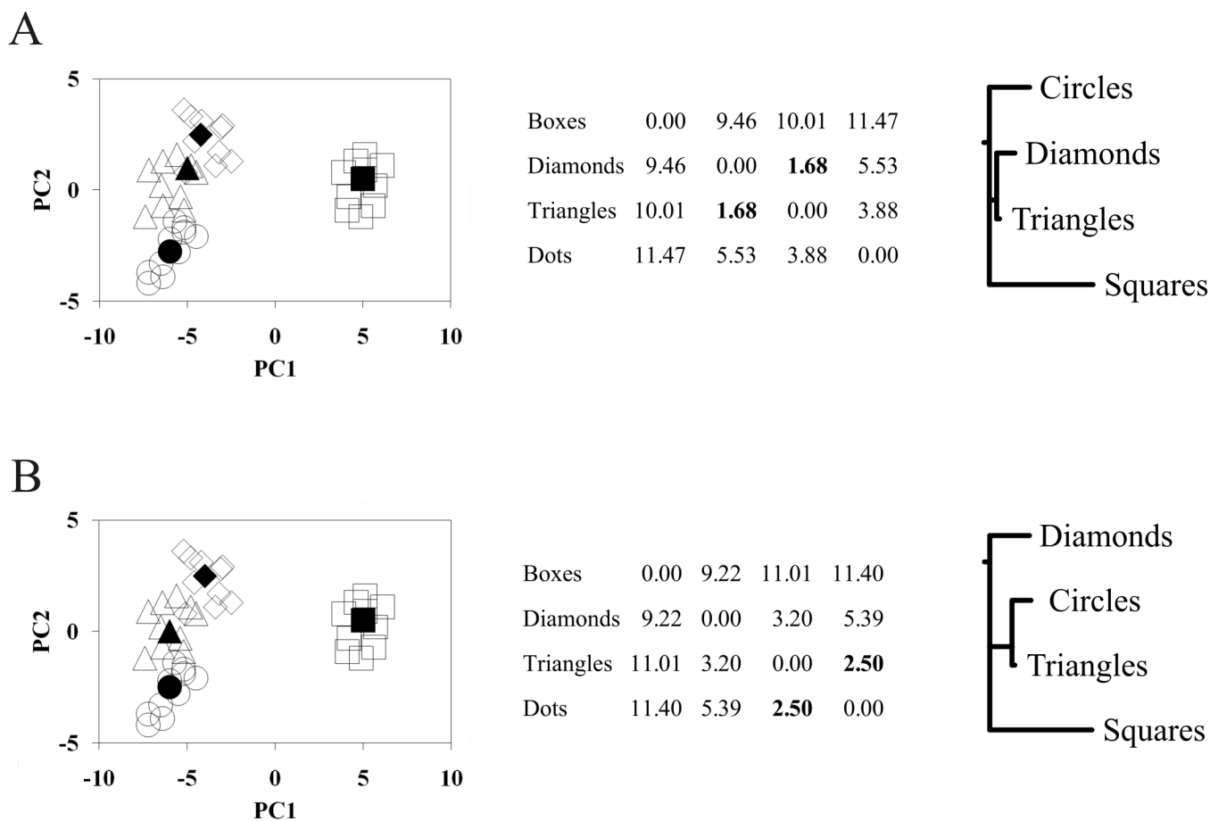
Figure 1. Examples of PC scores plots with the corresponding Euclidean distance matrices and metabolic trees. Open symbols represent simulated experimental data points. Closed symbols represent the cluster center positions calculated after random sampling of the respective datasets. Panel A presents the case where the centers of triangles and diamonds are closest together. Panel B presents the case where the triangles and circles have the smallest separation.
