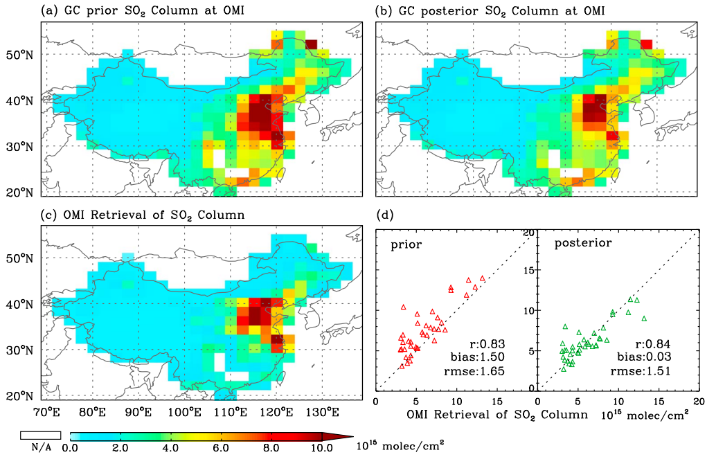
Figure 8. Same as Figure 7 but for comparison of the GEOS-Chem SO 2 simulation with OMI column SO 2 retrievals for the period of April 2008. The OMI planetary boundary layer (PBL) column SO 2 from the Level 3 daily products with 0.25° × 0.25° resolutions are aggregated into GEOS-Chem grid cells.
