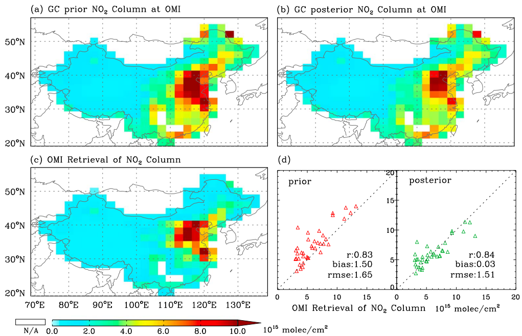
Figure 9. Same as Figure 7 but for comparison of the GEOS-Chem NO 2 simulation with OMI column NO 2 retrievals for the period of April 2008. The OMI tropospheric column NO 2 from Level 2 daily products with 0.25° × 0.25° resolutions are aggregated into GEOS-Chem grid cells.
