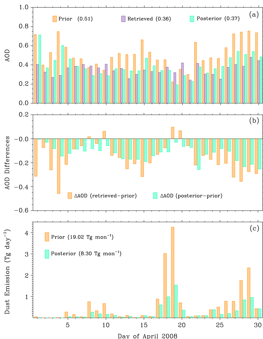
Figure 4. (a) Time series of the spatially averaged daily MODIS AOD retrievals (purple) for April 2008 over the Eastern China, compared by the prior (orange) and posterior (green) spatial averaged daily GEOS-Chem AOD that are sampled in the MODIS AOD tempo-spatial space. (b) Time series of the expected daily AOD adjustments (orange) that are the differences between MODIS AOD and the prior GEOS-Chem AOD and their real adjustments (green) that are the differences of posterior from prior GEOS-Chem AOD. (c) Time series of the prior (orange) and posterior (green) daily dust emissions over China for April 2008.
