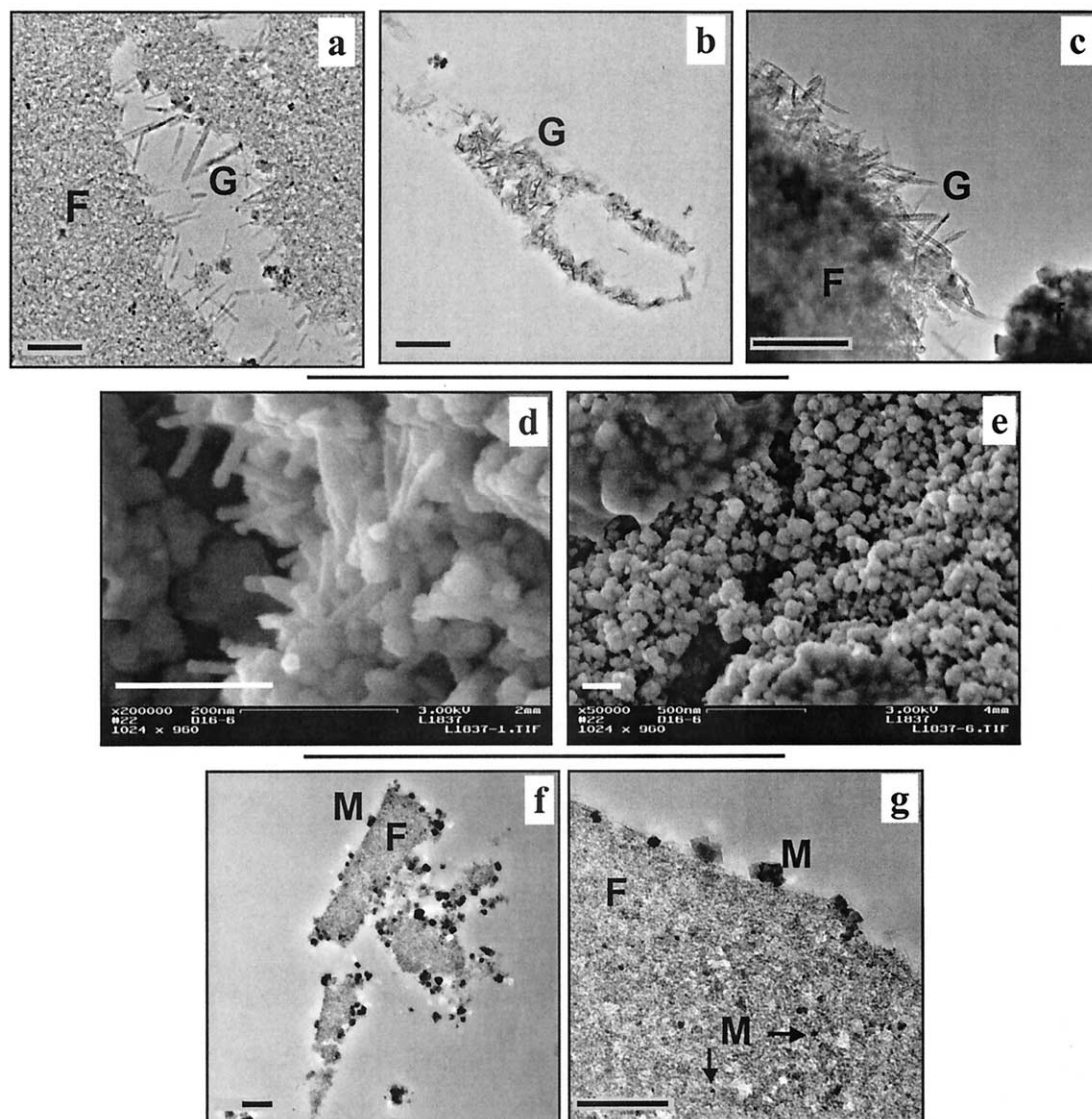
Fig. 7. TEM and SEM images of goethite and magnetite secondary phases. TEM images of goethite reveal (a) perpendicular goethite (G) laths to the ferrihydrite (F) surface (top of 2-d column), (b) an oblique cross-section through a goethite-encrusted bacterium (top 4-d column), and (c) whole-mount of two ferrihydrite grains, one encrusted in goethite (top 16-d column). SEM images of (d) goethite and (e) magnetite (M) display their bulk morphology and small particle size. Also illustrated are TEM images of magnetite precipitates originating from the ferrihydrite surface isolated from the effluent end of the 4 d. (f, g) Arrows in the TEM image point to small magnetite nucleation sites within the ferrihydrite. All images shown are representative of the samples as a whole. Scale bars are equal to 200 nm.
