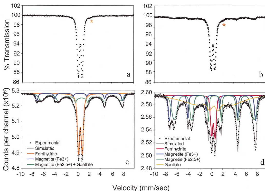
Fig. 6. Mössbauer spectrum of biomineralization solids from the (a) bottom (3 cm from inlet) and (b) top (3 cm from outlet) of the column reacted for 2 d and (c) middle (7 cm from inlet) and (d) top (3 cm from outlet) of the column reacted for 16 d. The high energy peak of the ferrous doublet for the samples from the 2 d column are denoted by “*.” The simulated fit (solid lines) to the experimental spectra (dotted) are shown for the column reacted for 16 d.
