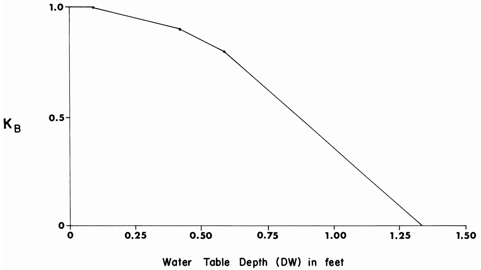
FIGURE 5. Depth of saturated water-table under sandbars and barren islands compared with evaporation rate ( K_B ).
