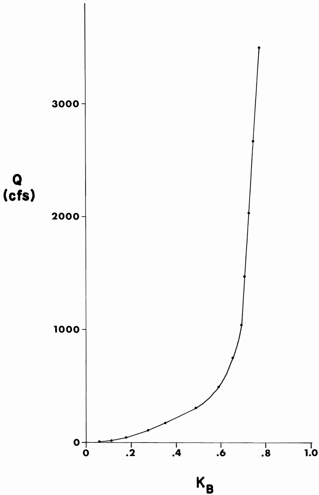
FIGURE 6. Evaporation rate from barren sand surface ( K_B ) at any discharge (Q).
