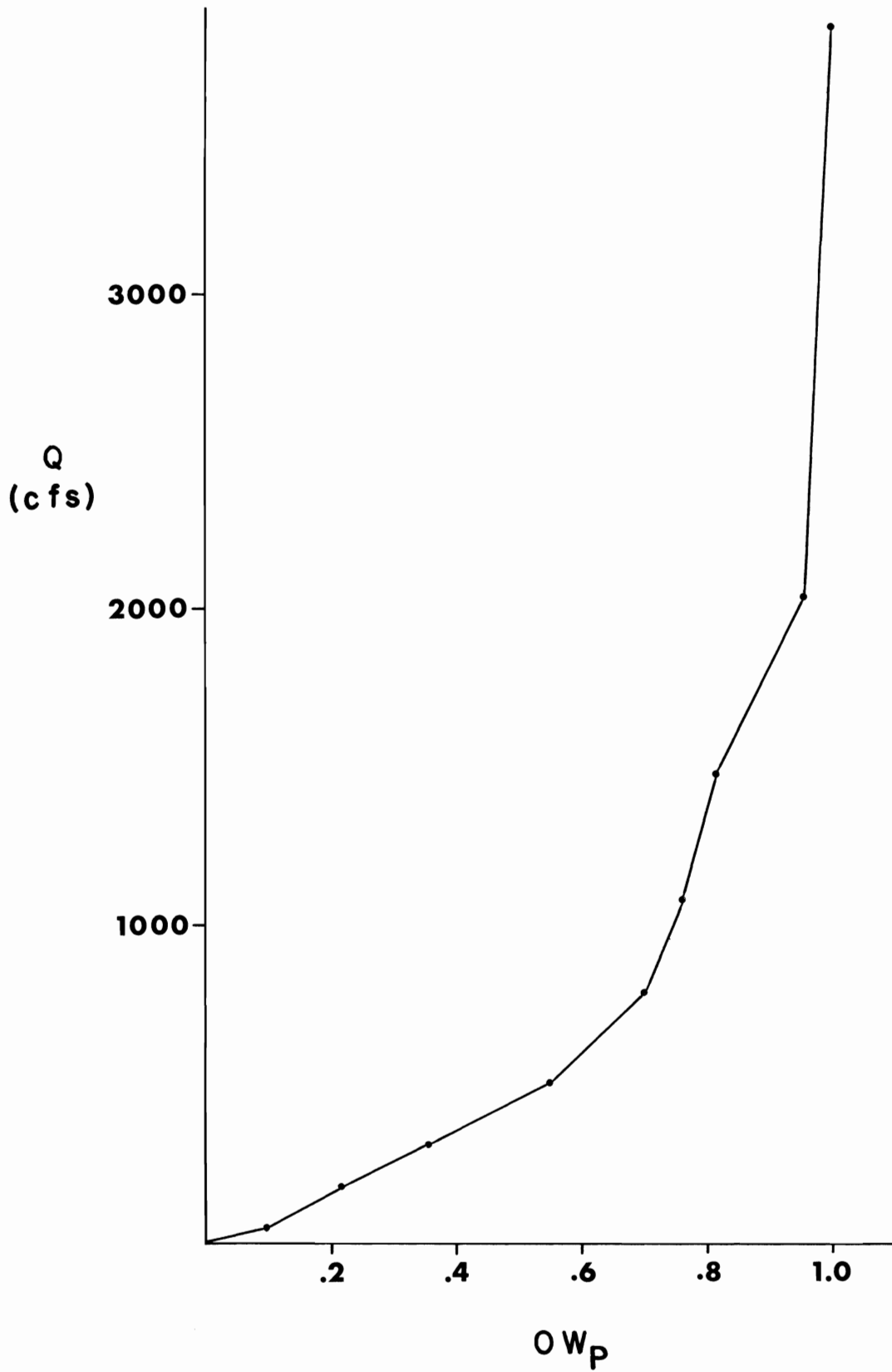
FIGURE 4. Proportion of total channel-width covered with water ( OW_p ) at any discharge (Q).
