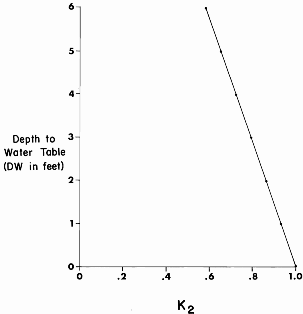
FIGURE 9. Depth to saturated water-table from soil surface as compared to K_2 .
