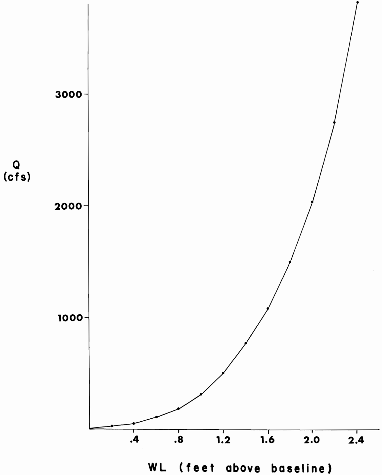
FIGURE 3. Relationship between water level (WL) above baseline elevation and discharge (Q) at Overton, Nebraska.
