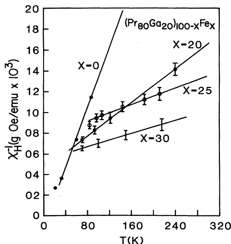
FIG. 12. Inverse high-field susceptibility for selected Pr glasses.
