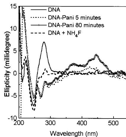
Figure 4. CD spectra of DNA, DNA + \text{NH}_4\text{F} , DNA-polyaniline (5 min), and DNA-polyaniline (80 min).
