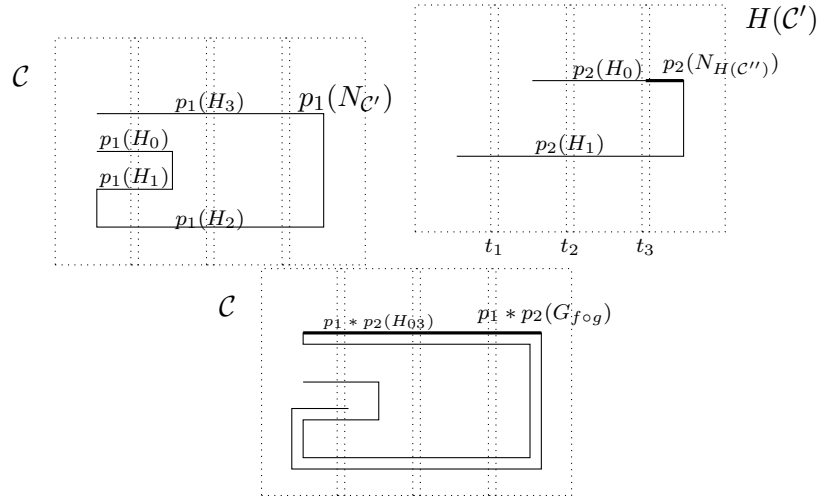
Figure 5.6: Composing permuted refinements. Here p_1 = (0 \ 2) and p_2 = (0 \ 1) are admissible. The top of p_1(N_{\mathcal{C}'}) is p_1(H_3) , so T_1 = 3 . The top of p_2(N_{H(\mathcal{C}'')}) is p_2(H_0) , so T_2 = 0 . Thus, the top of (p_1 * p_2)^{C_1}(G_{f \circ g}) is H_{T_2 T_1} = H_{03} (in bold).
