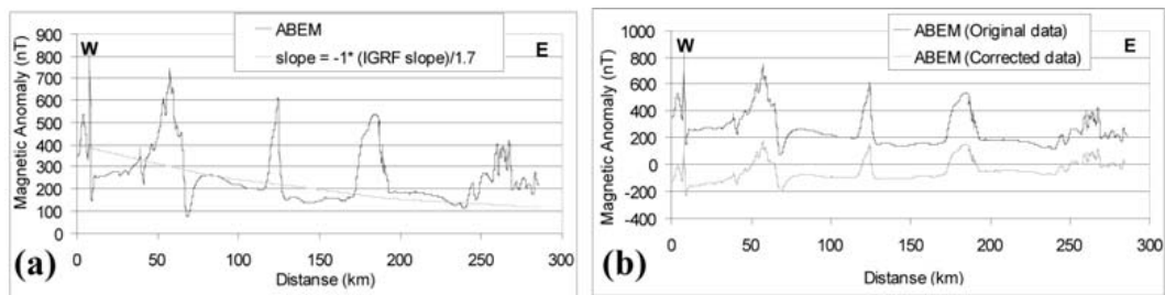
Fig. 5: (a) An E-W profile sliced from the ABEM data (Profile PB in Fig. 1). The trend line has been determined as per Fig. 3c. (b) The same profile before and after de-trending and re-scaling as per Fig. 3d.
