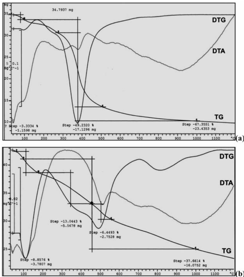
Fig. 4: TG/DTG/DTA diagrams of representative xylite (a) and matrix lignite (b) samples.
