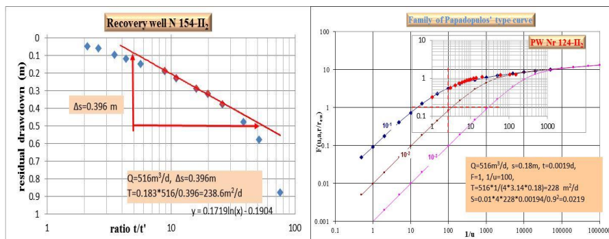
Figure 9 - Pumping test data of well Nr 154-P2 (Recovery and Papadopolos-Cooper's method respectively).
