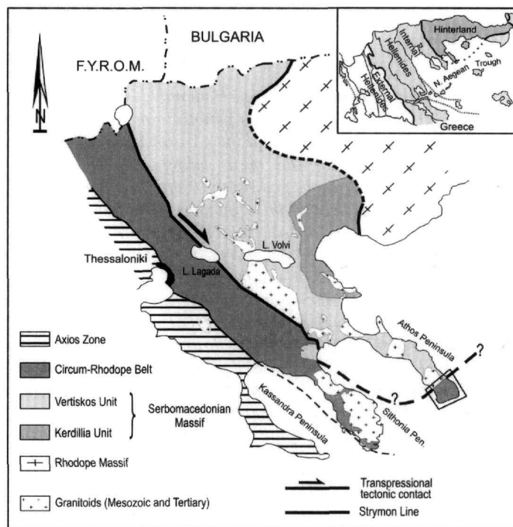
Figure 1 – Geotectonic map of central Macedonia-Chalkidiki peninsula
