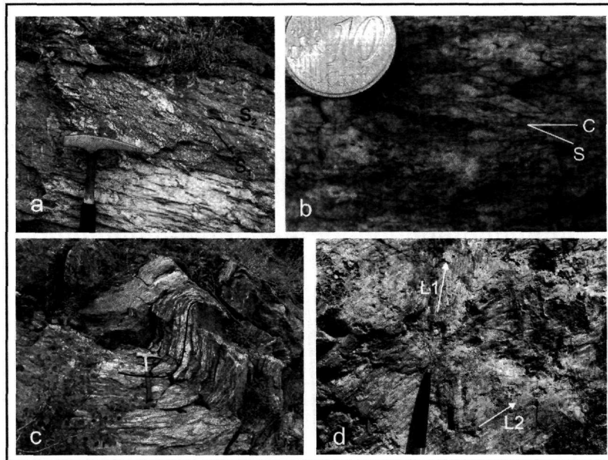
Figure 4 – Field photographs: (a) crenulation cleavage formed by the superposition of the S_2 foliation on the S_1 (b) S-C mylonitic fabric indicating left-lateral shearing in the green-gneisses, (c) asymmetric fold in the green-gneiss, (d) two generations of slickenlines (L1, L2) present on an E-W striking fault, with L2 (left-lateral strike-slip) overprinting L1 (reverse)
