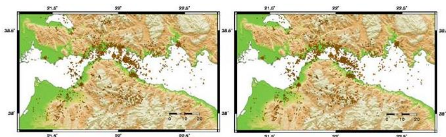
Figure 1 - Located seismicity ( M \geq 1.4 ) using regional 1-D velocity model (left) of Kaviris (2003) and the obtained local 1-D velocity model by the current study (right).
