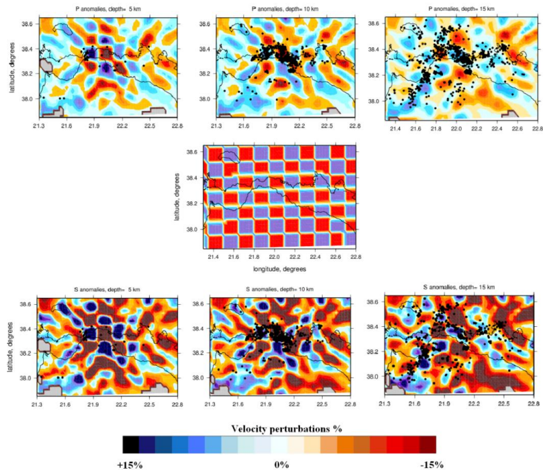
Figure 2 - Starting checkerboard anomaly distribution (central panel) and the resulting P- (upper panel) and S-velocity (lower panel) anomalies for the depth slices of 5, 10 and 15 km. The black dots indicate local earthquakes in the corresponding depth levels.
