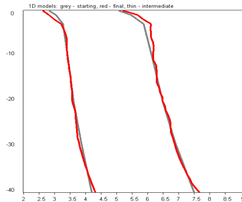
Figure 3 - Optimization results of the 1D velocity model (red line) setting as starting model the one obtained by the current study (grey line).
