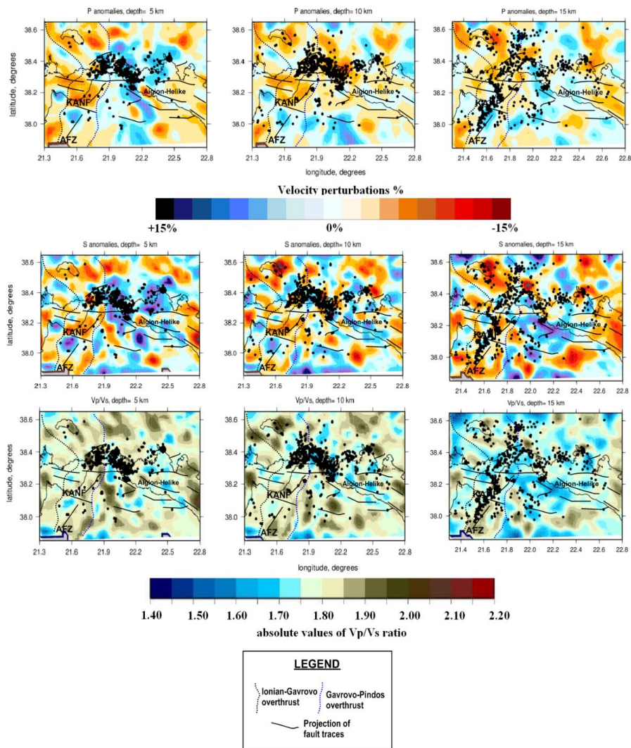
Figure 4 – Three dimensional distribution of P- (upper panel), S-velocity perturbations (central panel) and absolute Vp/Vs ratio (lower panel) for the depth slices of 5, 10 and 15 km.
