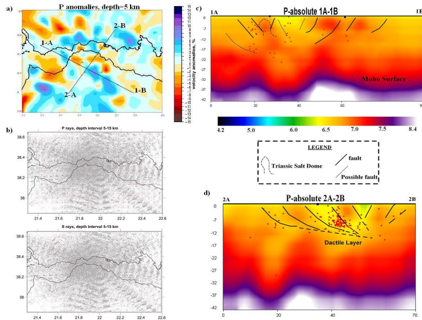
Figure 5 – a) Horizontal projection of the two profiles in NW-SE (1A-1B) and SW-NE (2A-2B) directions b) ray-path distribution of P and S waves c) Profile 1A-1B and d) Profile 2A-2B.
