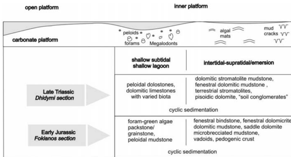
Fig. 7: Depositional settings of the Dhidymi and Fokianos sections.
