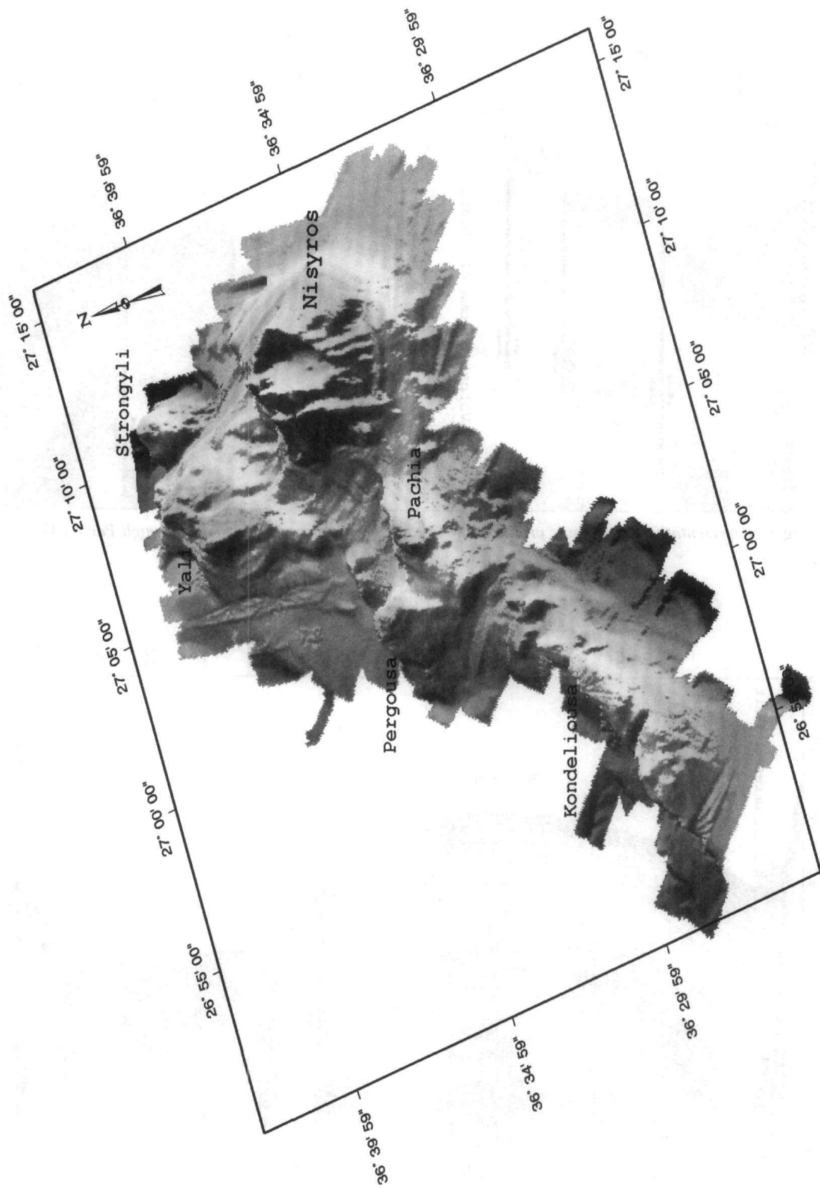
Fig 4: Perspective image of Nisyros and neighbouring volcanic islets. View from SW.
