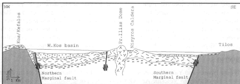
Fig 2a: Schematic tectonic profile through Kefalos-Nisyros-Tilos.
