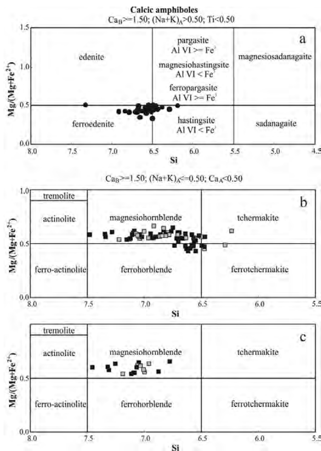
Figure 3 - Classification diagrams after Leake et al. (1997, 2003) a) Bi Hbl GRD, b) Bi-Hbl DR and Hbl DR, c) Hbl GRD; grey squares: sieved crystals, black squares: normal crystals.
