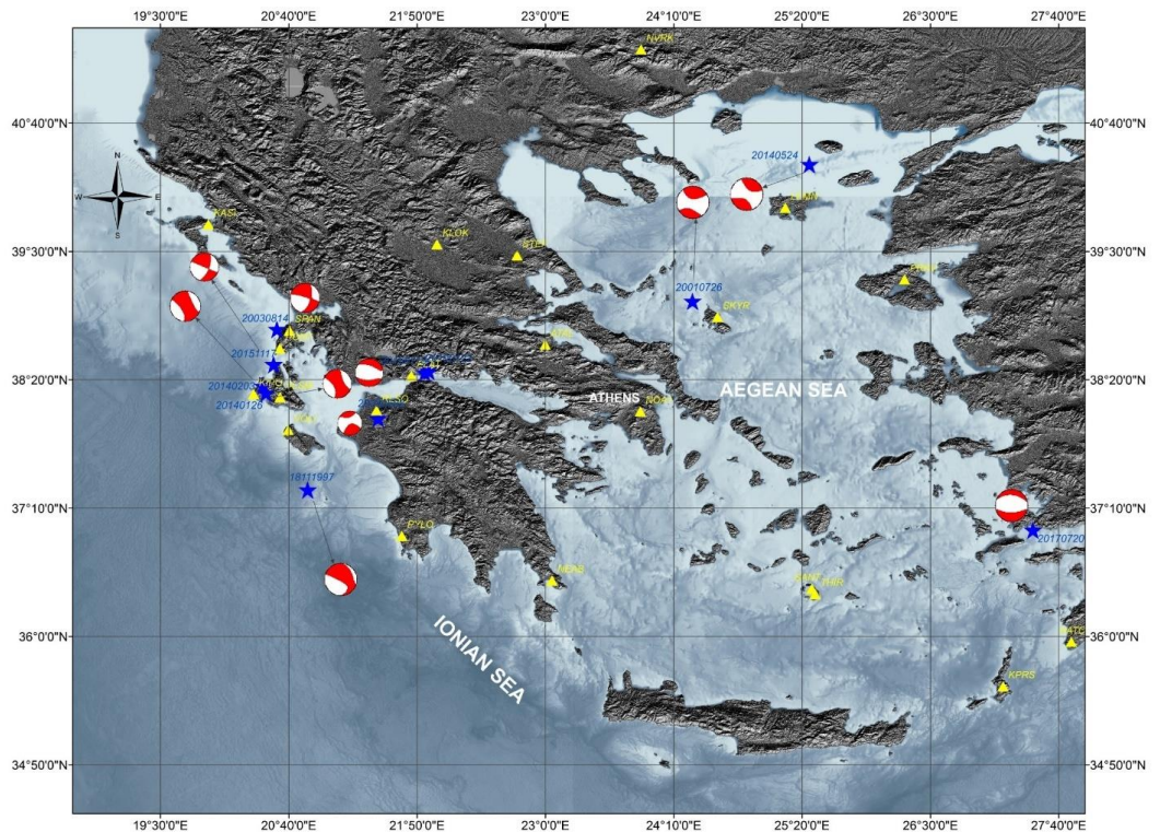
Fig. 1: Location map of Aegean seismic events (blue stars) with GPS records reported in this study. Beachballs indicate focal plane solutions (lower hemisphere, compressional quadrant in red colour) from moment Tensor inversion data ( http://www.globalcmt.org/CMTsearch.html ). We use EMOD bathymetry, and the ASTER GDEM for relief. Yellow triangles are NOANET stations. Illumination from SE.
