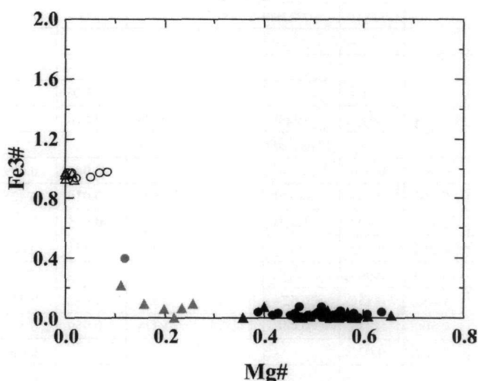
Figure 4 - Fe 3+ # vs. Mg# plot of the analysed Cr-spinels and their alteration products. Note the rapid increase in Fe 3+ # for ferrian chromite and Cr-magnetite (black, grey and open circles represent Cr-spinels, ferrian chromites and Cr-magnetites, respectively, from the area of Milia. Black, grey and open triangles represent Cr-spinels, ferrian chromites and Cr-magnetites, respectively, from the area of Pefki)
