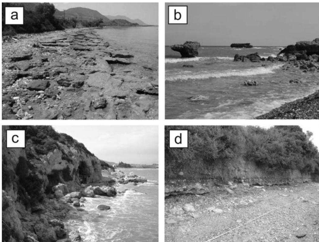
Fig. 5: (a) Uplifted and eroding beachrocks at Kalypso; (b) Uplifted (by 1 m asl) marine notch at Kynos; (c) Uplifted (approx. 2m asl) sea caves at Kynos; and (d) Eroding coastal alluvial cone at Alope. The base of this cliff consists of well cemented beach material, uplifted >1m asl since Roman times.
