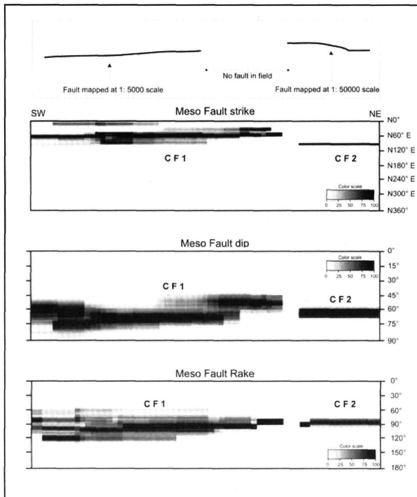
Figure 6 - Transect Analysis of the Corini Fault. Line brightness is proportional to the volume of data collected in the field. It can be seen that segment CF2 strikes N100°E, dips 60°-70° south and rake is almost 90°, i.e. motion is pure dip-slip. However, the rake along the segment CF1 is mostly > 90° indicating right-lateral movement
