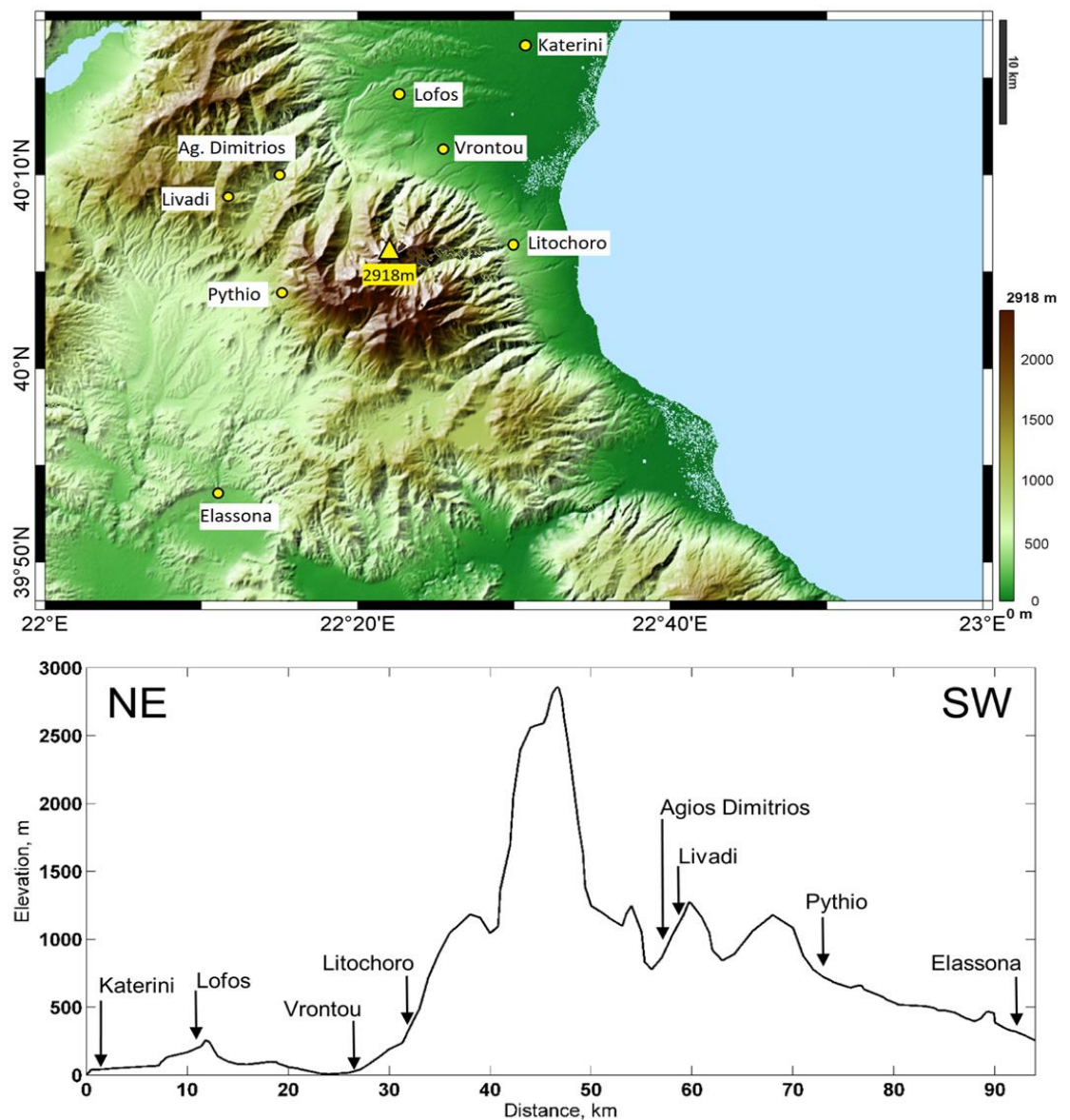
Fig. 2: SRTM topographic data image with the general setting of the study area (black rectangle Fig. 1), and the respective locations of the 8 meteorological stations ( upper panel ). ( lower panel ) The topographic transect considered in the study to assess the effects of orography on winter rainfall in the vicinity of Mount Olympus.
