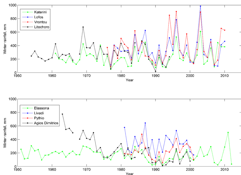
Fig. 3: Wintertime (DJFM) rainfall amounts for the stations along the eastern (marine) side of Mount Olympus ( upper panel ), and along the western (continental) side of the massif ( lower panel ).
