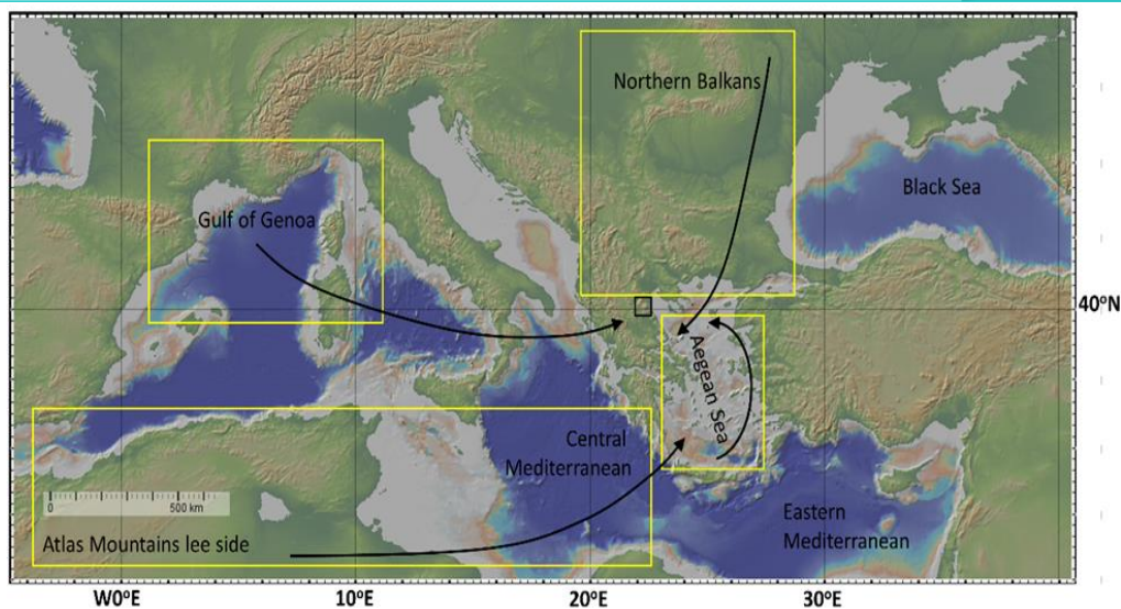
Fig. 1: Geographic location of the study area (black rectangle), in relation to the main cyclones' trajectories (black arrows) and areas of cyclogenesis (yellow rectangles) across the Mediterranean basin. Topographic and bathymetric background are provided by Geomapapp® ( http://www.geomapapp.org ; Ryan et al., 2009).
