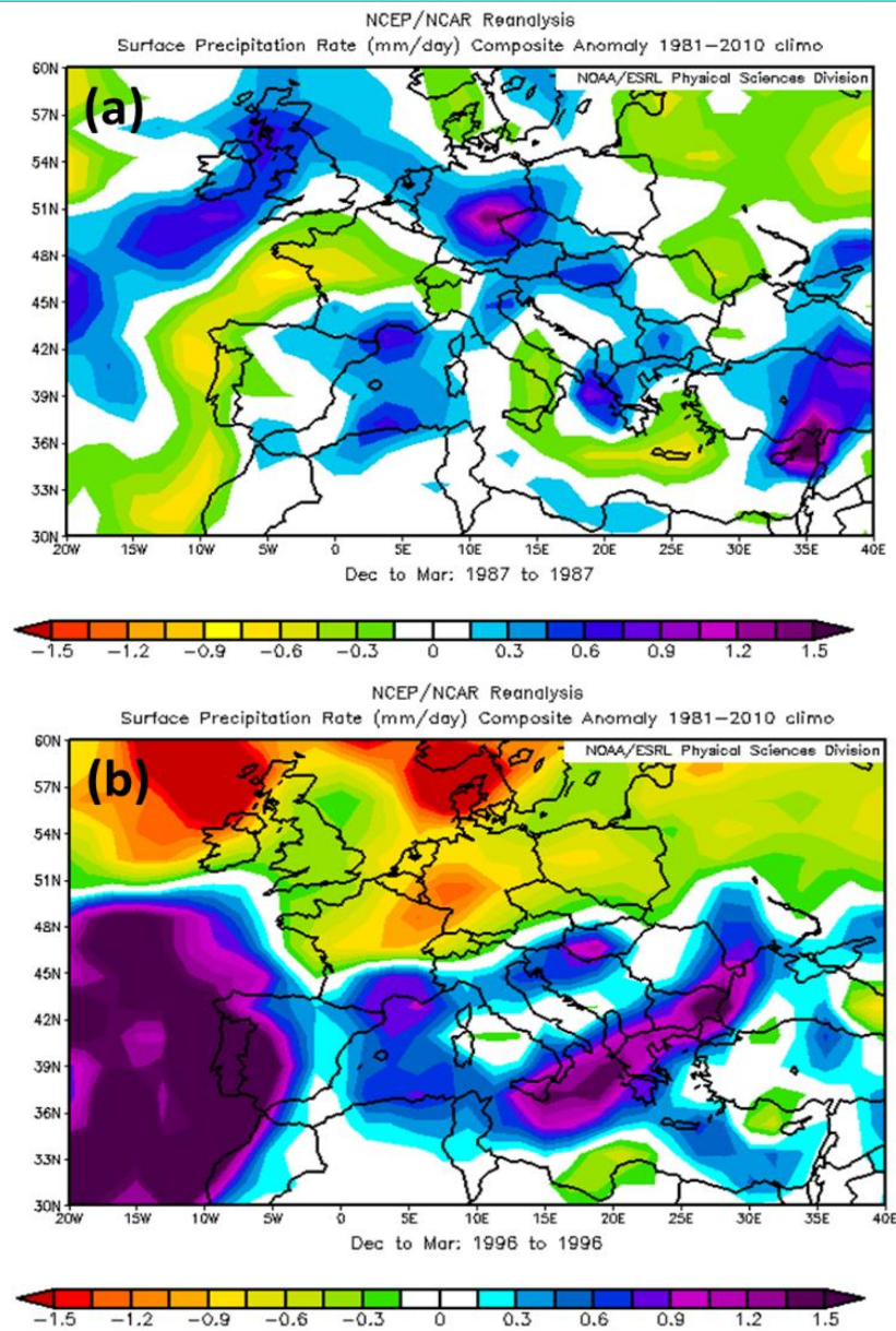
Fig.6: NCEP/NCAR surface precipitation anomalies from the 1981–2010 climatology for the winter of 1987 (a), with higher precipitation along the continental side of Mount Olympus and, (b) for the winter of 1996, when the marine side of Mount Olympus received the highest precipitation.
