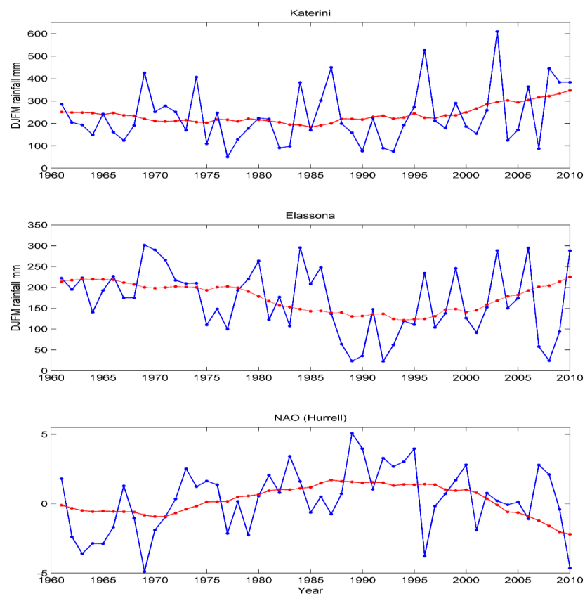
Fig.7: Interannual variability of winter rainfall in Katerini and Ellassona stations and the North Atlantic Oscillation Index. Red lines are the 8-year running means.
