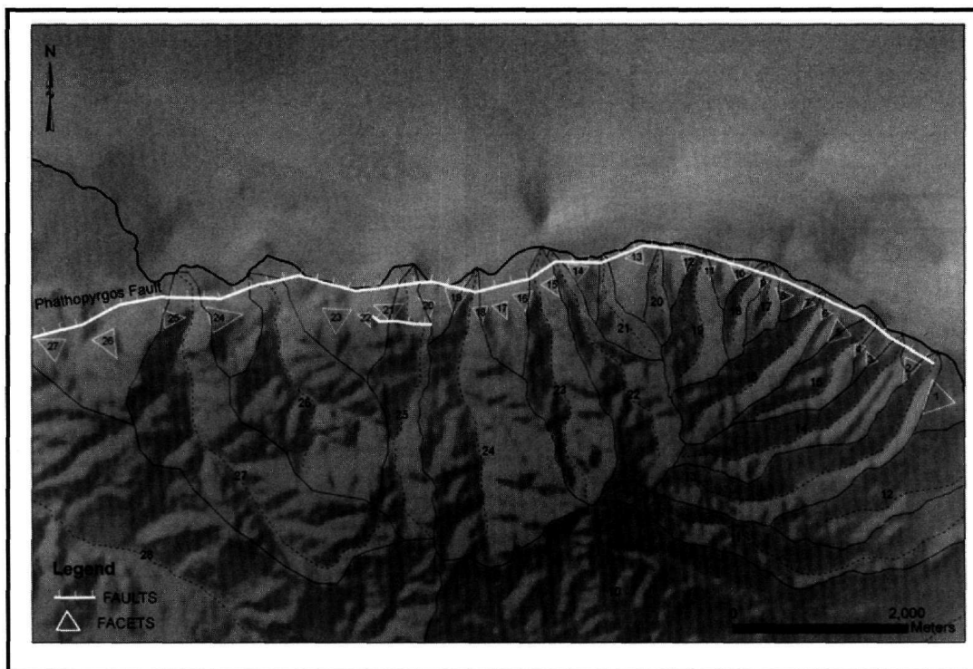
Figure 3 - Map of the Psathopyrgos fault area showing the catchments and triangular facets on its footwall. Integers inside triangles indicate facet numbering along strike
