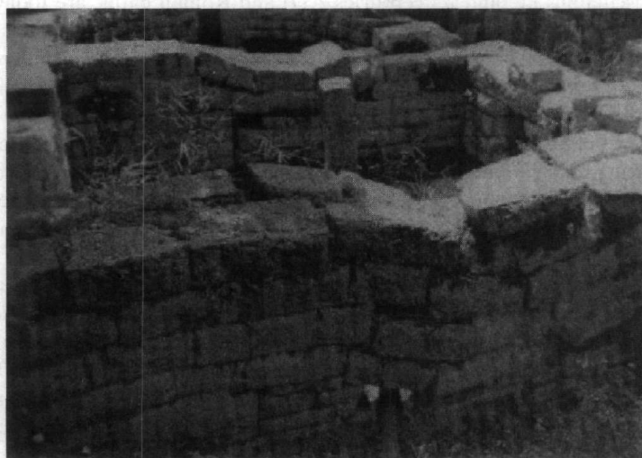
Fig. 7. The 4 th to 2 nd century BC Tower Gate (inner part). The most typical example of earthquake destroyed walls and foundation probably due directly to seismic fault activation, that is cracks (arrows) and tilted side (right) of the foundation.
