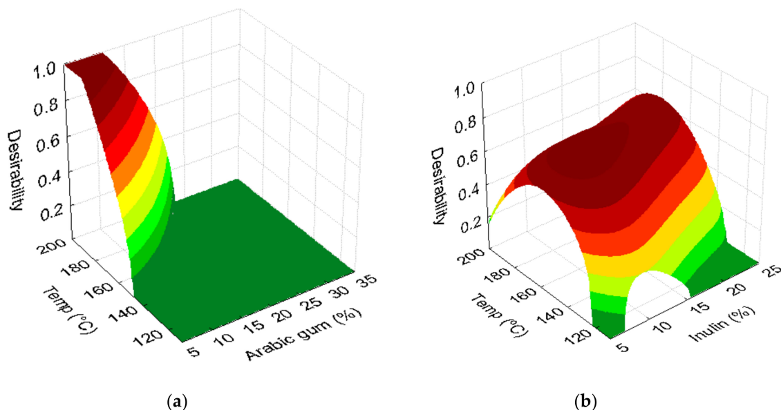
Figure 4. Desirability surface curves for optimal conditions: (a) Using EE and DY for arabic gum assays; (b) using EE, LC, and DY for inulin assays.
