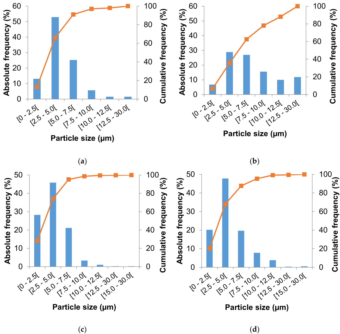
Figure 1. Relative frequency (Bars) and cumulative frequency (Line) equivalent to the diameter of microcapsules: (a) 5% AG, 155 °C; (b) 35% AG, 155 °C; (c) 5% inulin, 155 °C; (d) 35% inulin, 155 °C.
