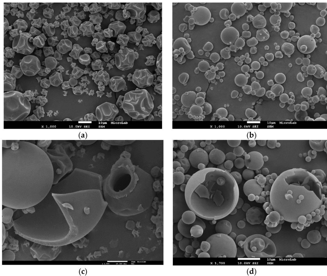
Figure 2. SEM images of microcapsules: (a,c) arabic gum (Magnification \times 1000 and \times 1500 ) and (b,d) inulin (Magnification \times 1000 and \times 1700 ).
