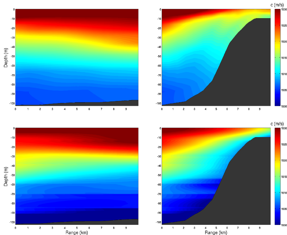
Fig. 3. (Color online) Sections of sound velocity calculated from temperature and salinity for the horizontal and vertical transects of Fig. 2 (left and right, respectively): ROMS predictions using the FORMS technique (top), and real data (bottom).
