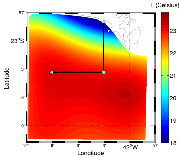
Fig. 2. (Color online) Range-independent (horizontal line) and range-dependent (vertical line) transects considered for forecasting: the circle indicates the position of the acoustic source, the background represents sea surface temperature.
