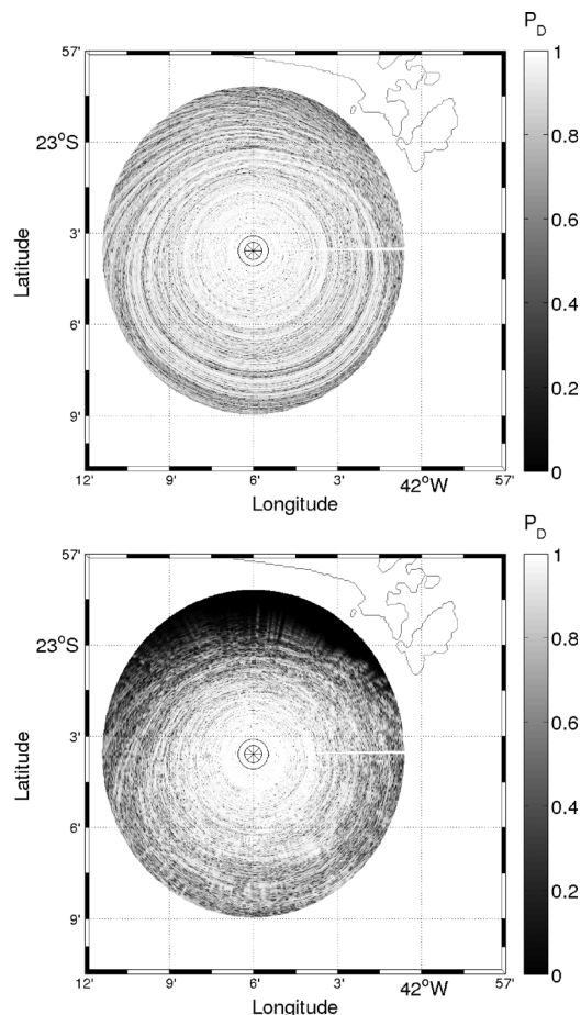
Fig. 4. Detection probability disks for a receiver at 9.5 m depth without upwelling (isovelocity case, top), and accounting for upwelling (bottom).
