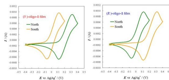
Figure 7. CV patterns for the achiral Fe(CN) 6 3- | Fe(CN) 6 4- redox couple, recorded
