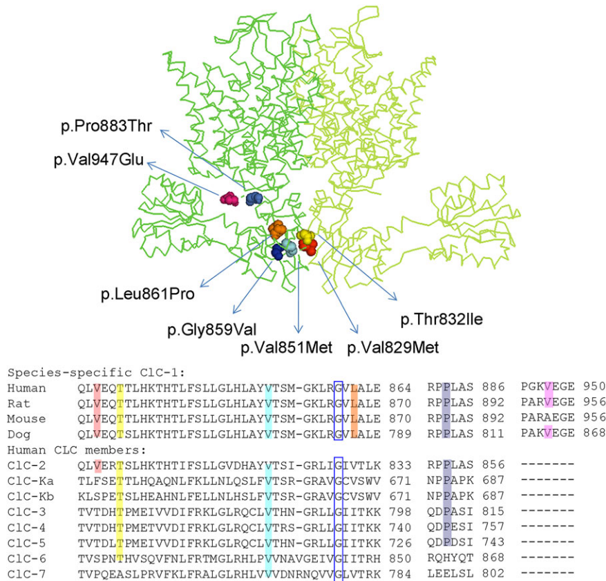
FIGURE 1 Structure and alignment of CLC channels. (A) Three-dimensional representation of hCLC-1 channel modeled upon the X-ray structure of an eukaryotic \text{Cl}^-/\text{H}^+ exchanger CmCLC (Feng et al., 2010) showing the localization of the C-terminal MC mutations. (B) Amino acid alignment of CLC proteins
