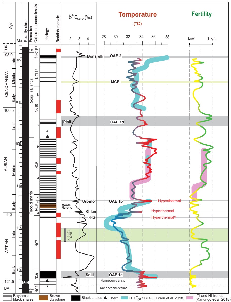
Figure 7. Synthesis of nannofossil-based nutrient (NI) and temperature (m-TI) variations reconstructed in the western Tethys as in Fig. 6. Nannofossil-derived SSTs (°C) are calibrated to TEX_{86}^H SSTs as in Fig. 6. Simplified TEX_{86}^H SSTs for ocean T > 15^\circ C (O'Brien et al., 2018) are reported in light blue. Middle Albian nannofossil TI and NI trends (pink lines) are from the Gault Clay Formation (Kanungo et al., 2018). Timescale is after Malinverno et al. (2010, 2012) for the late Barremian–Aptian and after the Geological Time Scale 2012 (Gradstein et al., 2012) for the Albian–Cenomanian.
