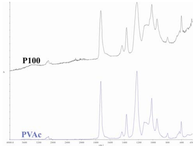
Fig.4. FT-IR spectrum of P100 compared with PVAc (polyvinyl acetate)
