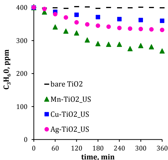
Figure 2. Acetone ( C^{\circ} = 400 ppm) degradation over time. Comparison between bare-TiO 2 and Me-doped TiO 2 by US assisted syntheses. Visible light irradiation (LED). Temperature constant at 25 °C. 40 % RH.
