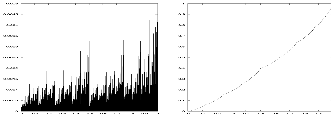
Fig. 2 Left: Histogram approximation of invariant measure \bar{\mu} (Lebesgue measure) of the IFSP in Example 1, Case 2. Right: Approximation to cumulative distribution function \bar{F}(x) of \bar{\mu} .
