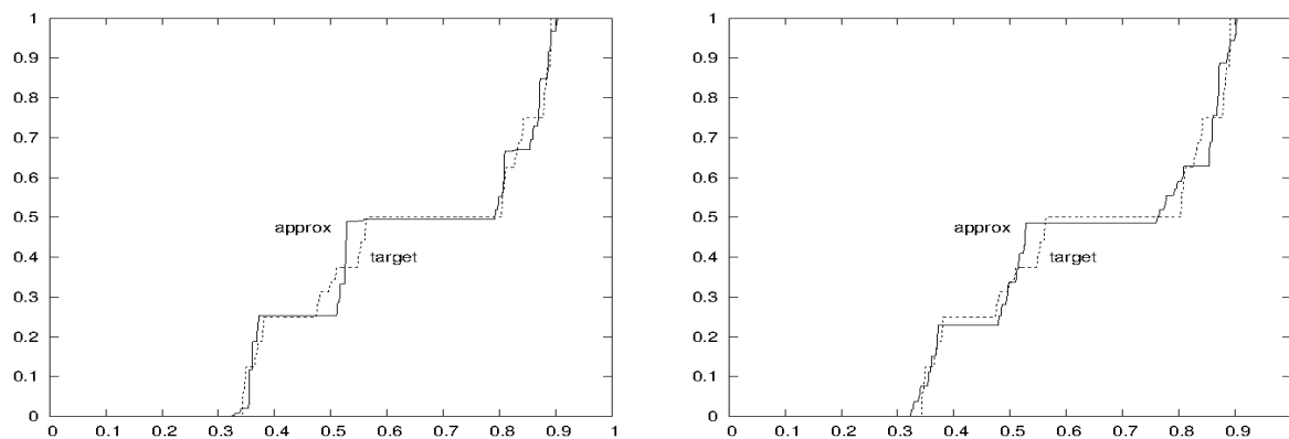
Fig. 8 Cumulative distribution functions for invariant measures of 8-map IFSPDP (left) and IFSP (right) from Table 4 which approximate the invariant measure \nu_\infty of the nonlinear dynamical system x_{n+1} = a_\infty x(1-x) . In each case, the CDF for the measure \nu is also shown for comparison.
