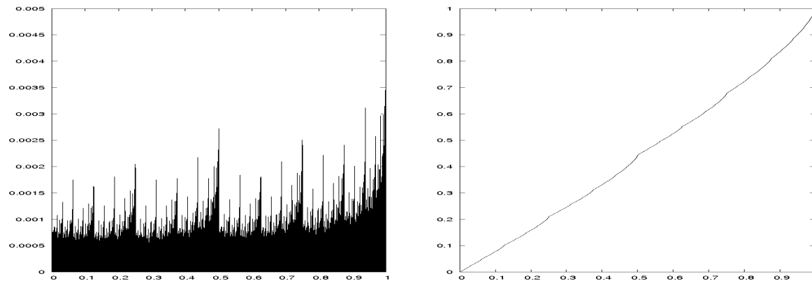
Fig. 3 Left: Histogram approximation of invariant measure \bar{\mu} of the two-map IFSPDP in Example 2, Case 1. Right: Approximation to cumulative distribution function \bar{F}(x) of \bar{\mu} .
