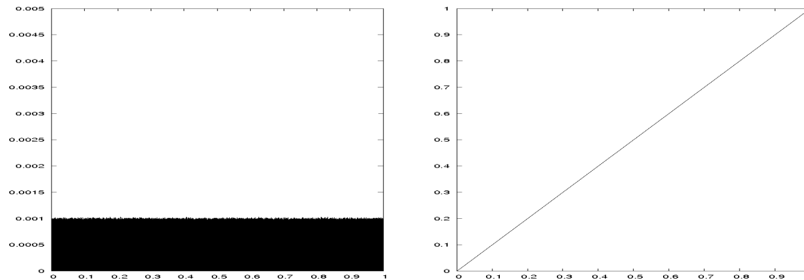
Fig. 1 Left: Histogram approximation of invariant measure \bar{\mu} (Lebesgue measure) of the IFSP in Example 1, Case 1. Right: Approximation to cumulative distribution function \bar{F}(x) of \bar{\mu} .
