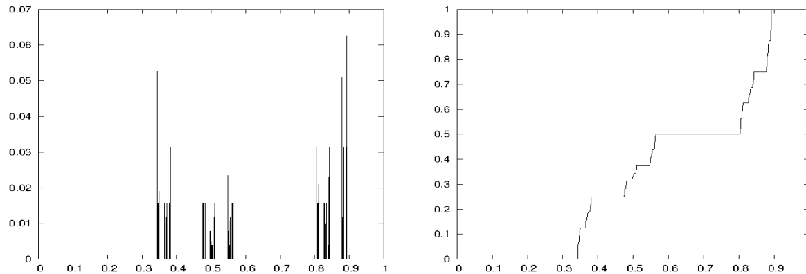
Fig. 7 Left: Histogram approximation of invariant measure \nu_\infty of the “ 2^\infty -cycle” chaotic attractor of the nonlinear dynamical system x_{n+1} = a_\infty x_n(1 - x_n) . Right: Associated cumulative distribution function F_\infty(x) .
