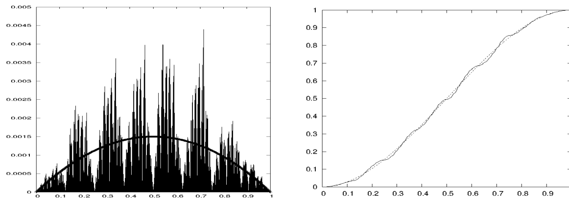
Fig. 5 Left: Histogram approximation of 14-map IFSPDP invariant measure \bar{\mu} (bottom left row of Table 1) using IFS wavelet-type maps of Eq. (36). The density function \rho(x) = 6x(1-x) of the target measure \nu is also plotted for comparison. Right: The cumulative distribution function (CDF) yielded by the histogram approximation to \bar{\mu} on the left. The CDF of the target, F(x) = 3x^2 - 2x^3 , is also plotted for comparison.
