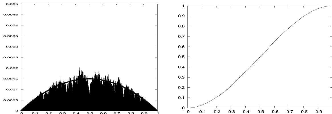
Fig. 6 Left: Histogram approximation of 14-map IFSPDP invariant measure \bar{\mu} (bottom row of Table 2) using IFS nonwavelet-type maps of Eq. (55). The density function \rho(x) = 6x(1-x) of the target measure \nu is also plotted for comparison. Right: The cumulative distribution function (CDF) yielded by the histogram approximation to \bar{\mu} on the left. The CDF of the target, F(x) = 3x^2 - 2x^3 , is also plotted for comparison.
