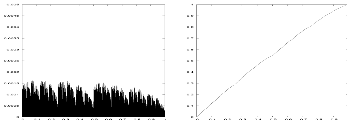
Fig. 4 Left: Histogram approximation of invariant measure \bar{\mu} of the IFSPDP in Example 2, Case 2. Right: Approximation to cumulative distribution function \bar{F}(x) of \bar{\mu} .
